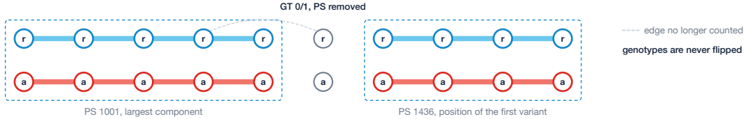
Supplementary Fig. 5: Window construction and phase-set update for the graph neural network. a , A window of \pm 20 variants (two allele nodes each) is opened around every phased variant with PE \geq 0.8 ; edges are the DOT edges with both endpoints in the window (blue and red arcs) plus self-loops; a dashed grey edge marks a cross-haplotype link. Predictions are read only in the central zone. b , Bridge-vertex feature: a variant whose removal disconnects the window graph. c , Definition of the central zone. A window holds at most 41 variants and 82 allele nodes (a 256-node cap exists but is never reached at the default window size); SNV, indel, SV and 5mC records are merged and sorted by position before nodes are created. Because offsets are normalized by the largest offset in the window, r_{\max} = 1 in practice and the retained zone is the central half of the window's genomic span. The same rule, with the same constant, defines which labelled nodes carried a training loss, so the zone scored at inference is the zone the network was trained on. Edges are the DOT edges with both endpoints in the window, symmetrized, plus one self-loop per node whose features are the mean over that node's incident edges. The predictions of the two allele nodes of a variant are averaged, and a variant covered by several windows receives the mean over those windows. d , The exported phasing graph (DOT) that the module reads: one line per voting pair, source and target written as position.allele, and the vote weight accumulated at the source as the label. e , Phase-set update, before correction: a variant with predicted error probability \geq 0.30 (amber) inside a phase set. f , After correction the variant is written as an unphased genotype without PS; connectivity of the remaining variants is recomputed over the surviving DOT edges, the largest component keeps the original PS and every other component receives a new PS equal to the position of its first variant. Genotypes are never flipped.
