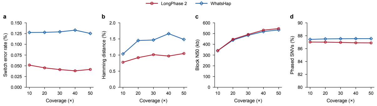
Figure 5: Phasing of PacBio HiFi data compared with WhatsHap. HG002 PacBio HiFi (Revo) reads down-sampled to 10–50 \times , one replicate per coverage[ state whether one call set was used for every coverage ]; SNV-only phasing scored against v5.0q; LongPhase 2 uses the network trained on nanopore data. Panels as in Fig. 2a–d. a , Switch error rate. b , Block-wise Hamming distance. c , Phase-block N50. d , Fraction of benchmark heterozygous SNVs phased.
