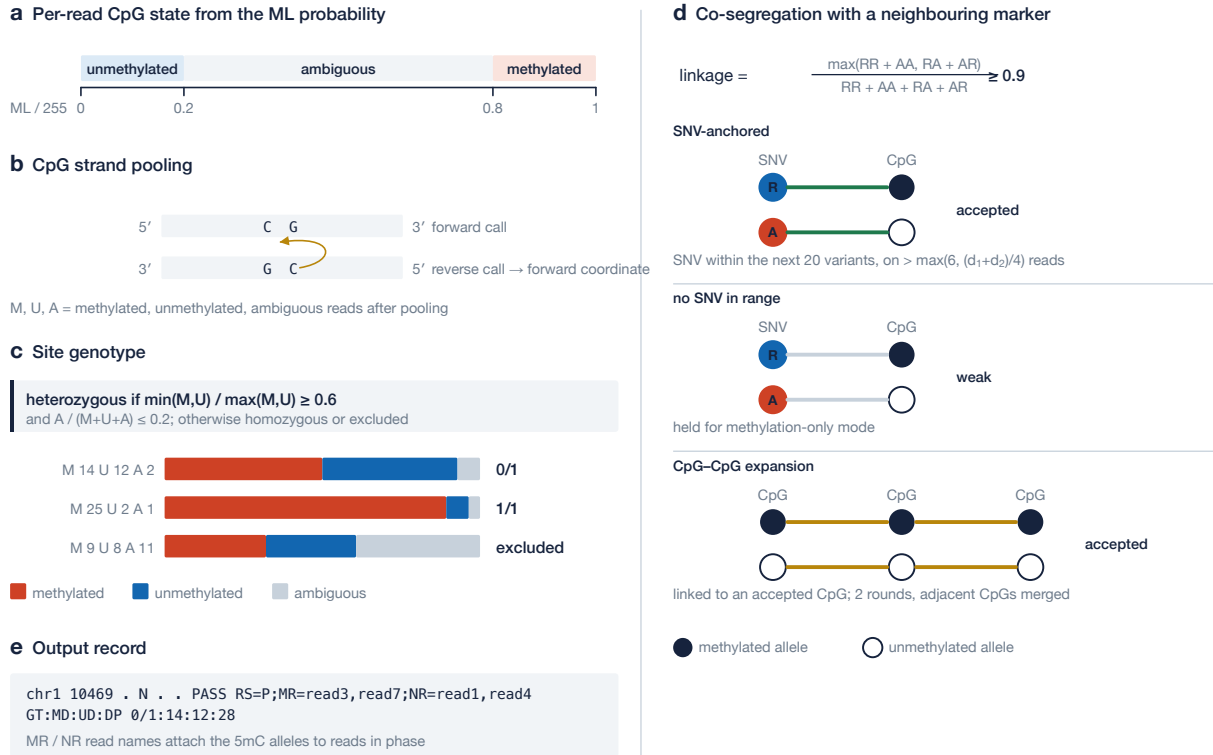
Supplementary Fig. 9: Allele-specific methylation calling with modcall. a , Per-read CpG states from the ML probability: methylated \geq 0.8 , unmethylated \leq 0.2 , otherwise ambiguous. Only CpG dinucleotides are considered. b , Reverse-strand calls are mapped to the forward CpG coordinate and the two strands are pooled, so that a CpG is genotyped once from all reads covering it. c , A site is called heterozygous when \min(M_R, U_R) / \max(M_R, U_R) \geq 0.6 and A_R / (M_R + U_R + A_R) \leq 0.2 , where M_R , U_R and A_R are methylated, unmethylated and ambiguous read counts. d , Balance alone does not imply allele specificity, since stochastic methylation satisfies the same inequalities. Candidates are therefore required to co-segregate with a neighbouring marker at linkage ratio \max(RR + AA, RA + AR) / (RR + AA + RA + AR) \geq 0.9 , in SNV-anchored mode against an SNV within the next 20 variants, or in methylation-only mode against another candidate CpG where no informative SNV is in range. Weakly connected CpGs are admitted by iterative expansion against already accepted CpGs. e , Output record with methylated and unmethylated read names used by phase . [Four real-data panels exist in the group's thesis and slide material and would replace assertion with evidence throughout this figure. (i) Per-site scatter of ML probability at heterozygous versus homozygous CpGs with the 0.8 and 0.2 lines marked, justifying both thresholds and showing that it is the homozygous sites that spread across the ambiguous band; the original was computed on 48 sites in the imprinted SNRPN locus, which is too small and too special a sample to stand in a Nature Methods supplement — recompute genome-wide on HG002. (ii) Distribution of the linkage ratio \max(P, Q) / (P + Q) stratified by the true class of the site pair (heterozygous-heterozygous, homozygous-homozygous, heterozygous-homozygous). This is the strongest justification available for the 0.9 threshold, because in the original the three classes separate (roughly 0.65–1, 0.5–0.75 and 0.5–0.7), showing that the cut removes homozygous sites misclassified as allele-specific rather than being an arbitrary round number. (iii) Alignment views of an accepted and a rejected candidate under the two-strand CpG criterion in b . (iv) A low-coverage example showing the \max(6, (n_1 + n_2)/4) span requirement terminating a scan. Regenerate all four with the submitted version on the data used in this paper.]
