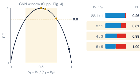
Supplementary Fig. 2: Pairwise allele support, weighted voting and phasing entropy. a , Between two variants u and v the reads accumulate four weights ( w_{rr}, w_{ra}, w_{ar}, w_{aa} ), each read adding 1 when both bases have quality \geq Q12 and 0.1 otherwise. P = w_{rr} + w_{aa} and Q = w_{ra} + w_{ar} are the supports for the two possible pairings and s = \min(P, Q) / \max(P, Q) their ambiguity. b , The pair votes for the better-supported pairing: at weight 20 when s \leq 0.1 with P + Q \geq 1 or, irrespective of s , when one pairing has less than 1 unit of support and the other at least 1; at weight 1 otherwise; and not at all when s > 0.7 (0.3 for SNV-5mC pairs, which also cast no vote when P + Q < 1 ). A voting variant that is a tandem-repeat indel votes at weight 0.1. The vote names a haplotype for v relative to the haplotype already assigned to u . c , Variant v receives weighted votes from up to k = 35 upstream variants that share a read with it, at any distance; line thickness encodes vote weight. The weighted totals h_1 and h_2 decide the haplotype; a tie opens a new phase block. d , Guard against a single erroneous ultra-long read: among the votes received by v , those resting on a single read ( P + Q \leq 1 , amber) are counted, and if more than three exist, h_1 and h_2 are recomputed from the votes with s < 0.2 , weight \geq 1 and a non-indel voter only. e , Phasing entropy of the vote totals, PE = -\sum_i p_i \log_2 p_i with p_i = h_i / (h_1 + h_2) , as a function of the vote split (left) and for four examples (right); values \geq 0.8 (shaded) open a window for the neural network (Supplementary Fig. 4). PE, h_1 and h_2 are written to the VCF as INFO/PE, INFO/H1 and INFO/H2. f , Block formation. Variants are visited in coordinate order; a variant whose next heterozygous variant lies more than 300 kb away ( -distance ) is skipped and casts no votes, a variant that receives no informative vote or a tie (amber) starts a new phase set when it lies beyond the last position reached by an accepted edge and is otherwise left unphased, and blocks holding a single variant are dropped (grey). Haplotype labels propagate along the block as the phased genotypes 0|1 and 1|0; the phase set (PS) is the position of its first variant.
