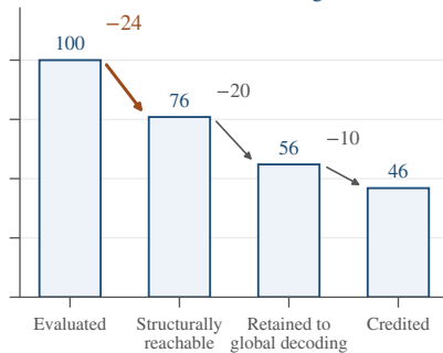
MedCaseReasoning
