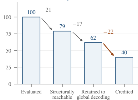
DiagnosisArena
