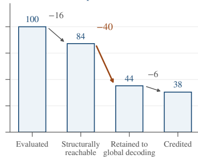
Open-XDDx
