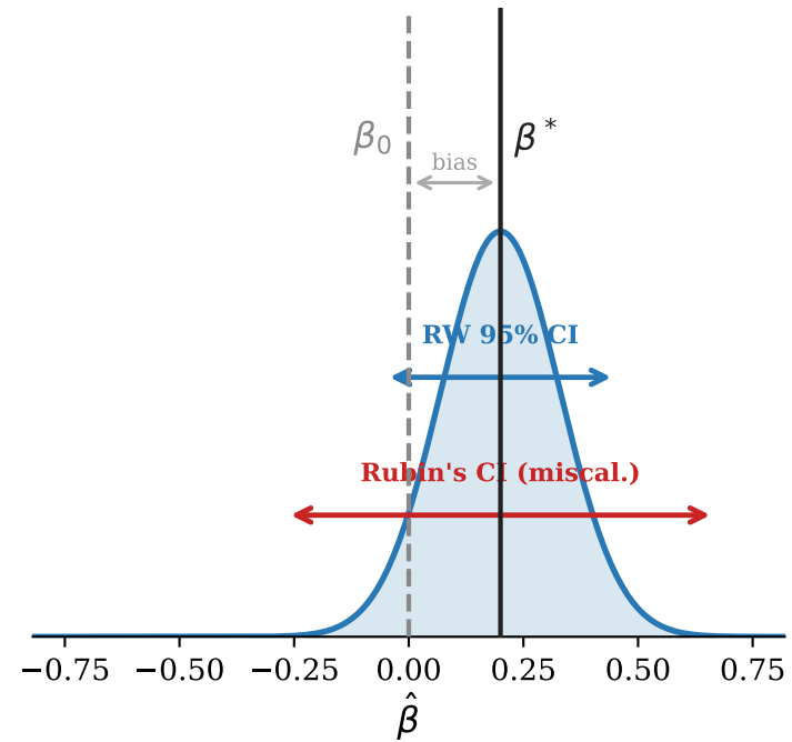
(c) Uncongenial — conservative
