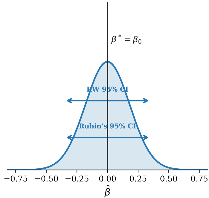
(a) Congenial imputation
