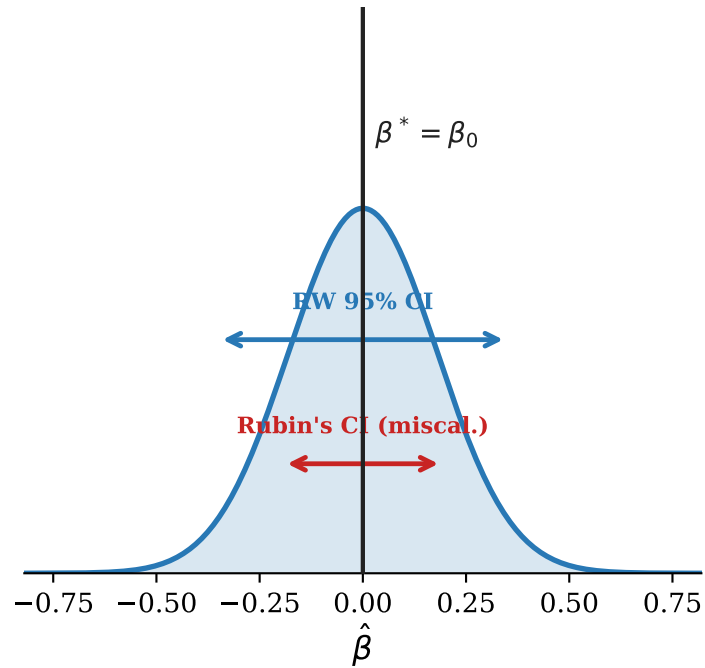
(b) Uncongenial — anti-conservative
