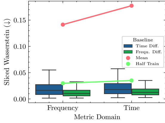
(a) ECG.
