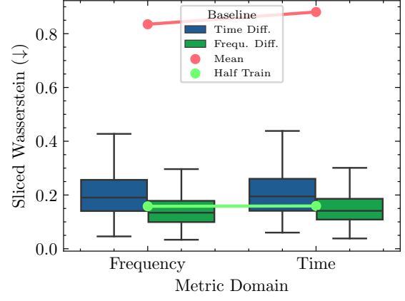
(b) MIMIC-III.
