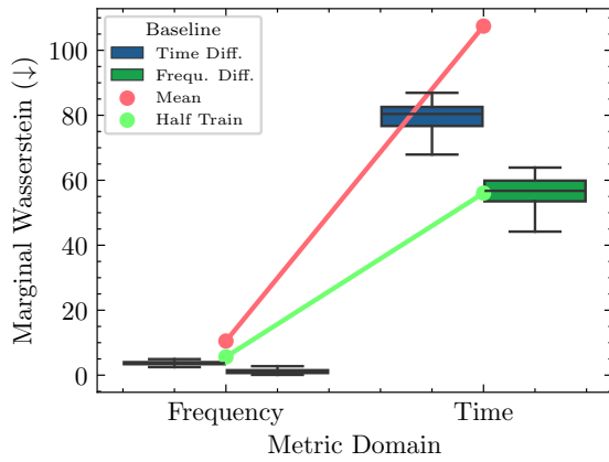
(e) NASA-Discharge.
