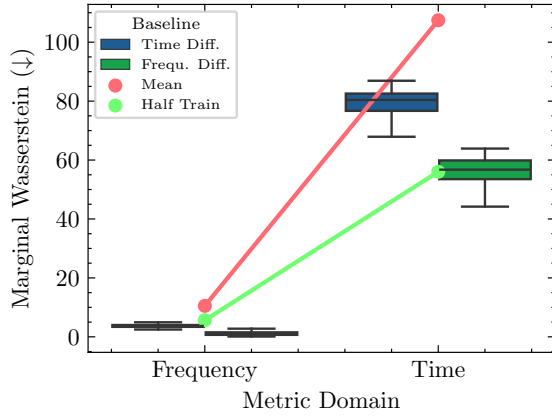
(c) NASDAQ-2019.
