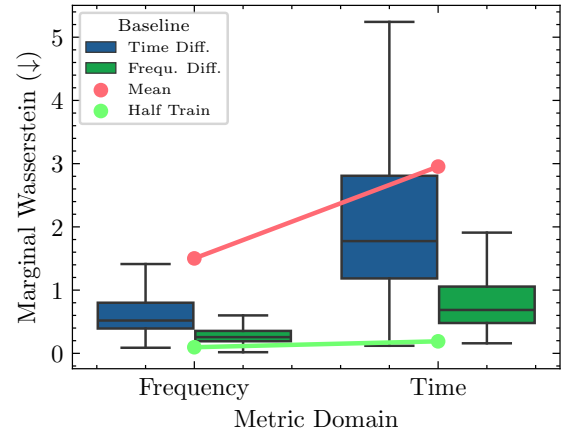
(f) US-Droughts.
