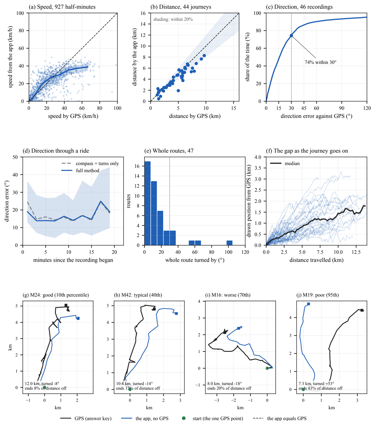
Figure 2. Motorcyclist, with the phone in a trouser pocket. (a) Speed per half-minute against GPS; the line is the middle of each 10 km/h band, the shading the middle half, and on the dashed line the two agree. (b) Distance per journey of at least 1 km; the shading is within 20%. (c) How often the direction is within a given angle of GPS. (d) Direction error through a ride, in two-minute bins with at least 300 graded seconds: the full method against the compass heading with the angle from turns alone. (e) How far each whole route is turned. (f) How far the drawn position is from GPS as the journey goes on: one thin line per route, and the median. (g–j) Four routes at the 10th, 40th, 70th and 95th percentile of end drift, labelled as in Appendix A; each is turned together with its GPS track by an arbitrary angle so as not to show where it was recorded.
