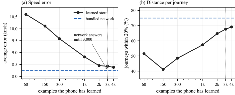
Figure 6: A phone that has learned only a few examples, against the built-in network. The store was tested holding 60 to 4000 examples; the network was measured only on recordings it had never seen. The dotted line is where the app hands over from the network to the store.
