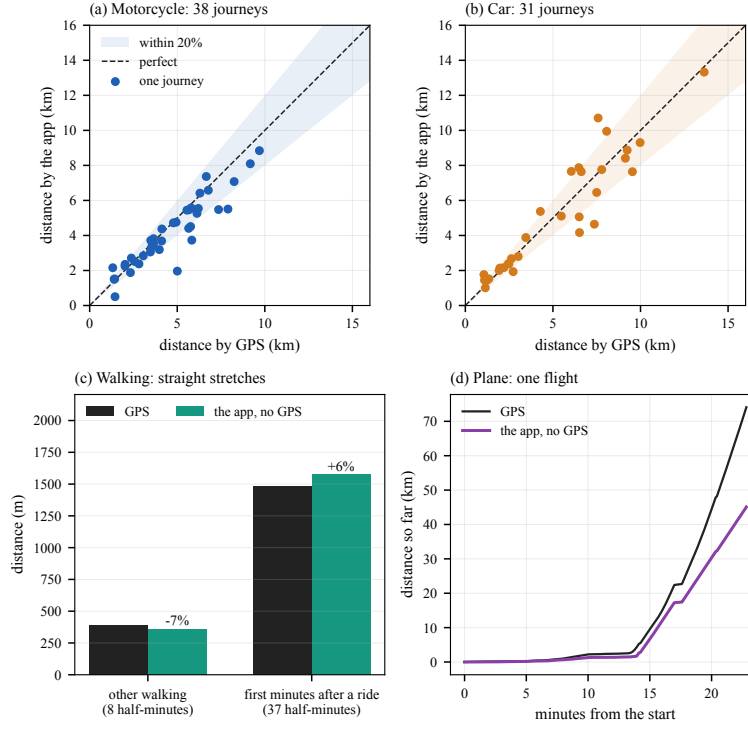
Figure 2: Distance by the app against GPS. (a, b) Each dot is one journey with at least 1 km that GPS could check; the shading is within 20%. (c) Straight stretches of walking, added up. (d) Distance so far on one flight.
