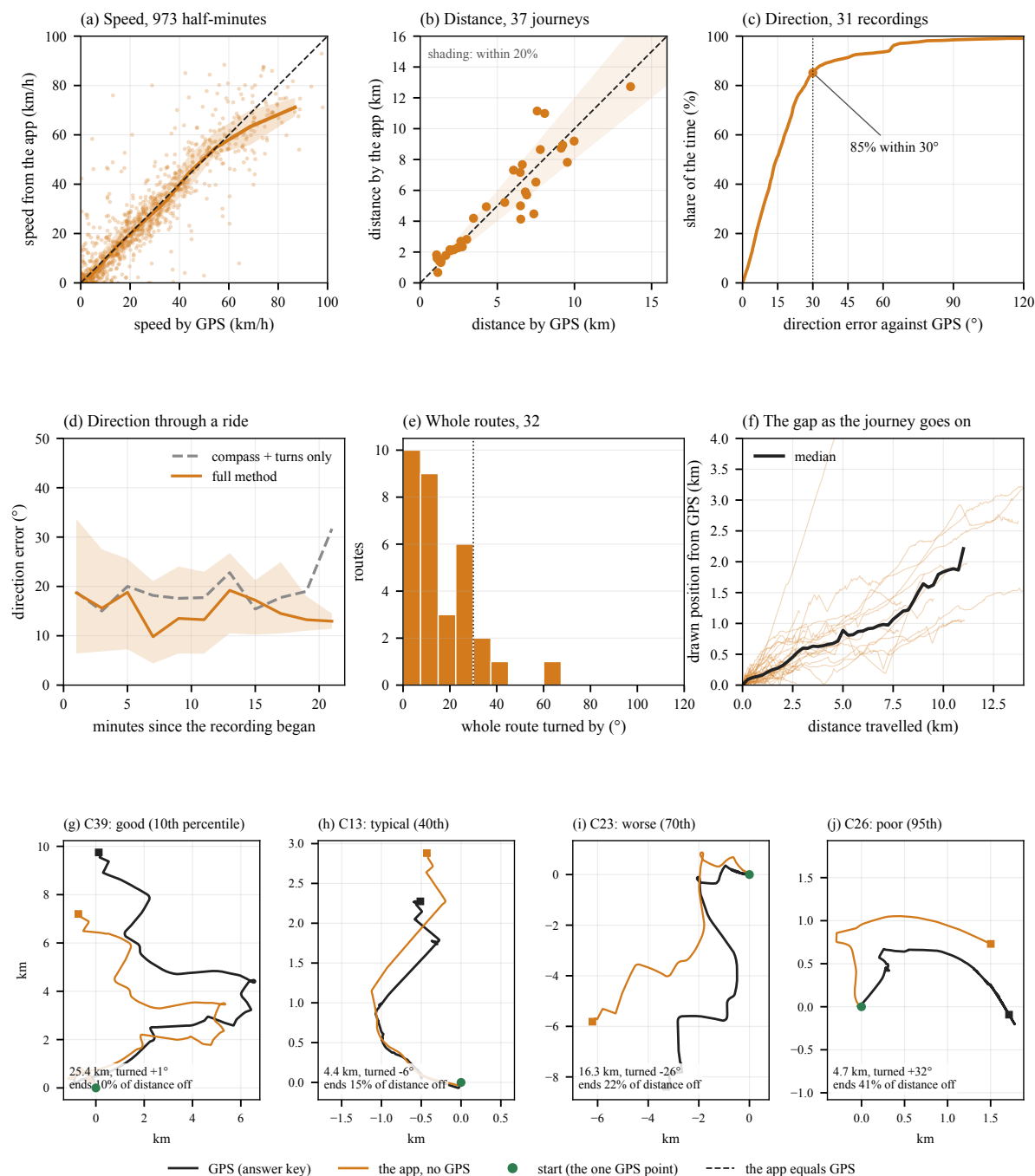
Figure 4. Car, with the phone in a pocket, lying flat or in a mount. (a) Speed per half-minute against GPS; the line is the middle of each 10 km/h band, the shading the middle half, and on the dashed line the two agree. (b) Distance per journey of at least 1 km; the shading is within 20%. (c) How often the direction is within a given angle of GPS. (d) Direction error through a ride, in two-minute bins with at least 300 graded seconds: the full method against the compass heading with the angle from turns alone. (e) How far each whole route is turned. (f) How far the drawn position is from GPS as the journey goes on: one thin line per route, and the median. (g–j) Four routes at the 10th, 40th, 70th and 95th percentile of end drift, labelled as in Appendix A; each is turned together with its GPS track by an arbitrary angle so as not to show where it was recorded.
