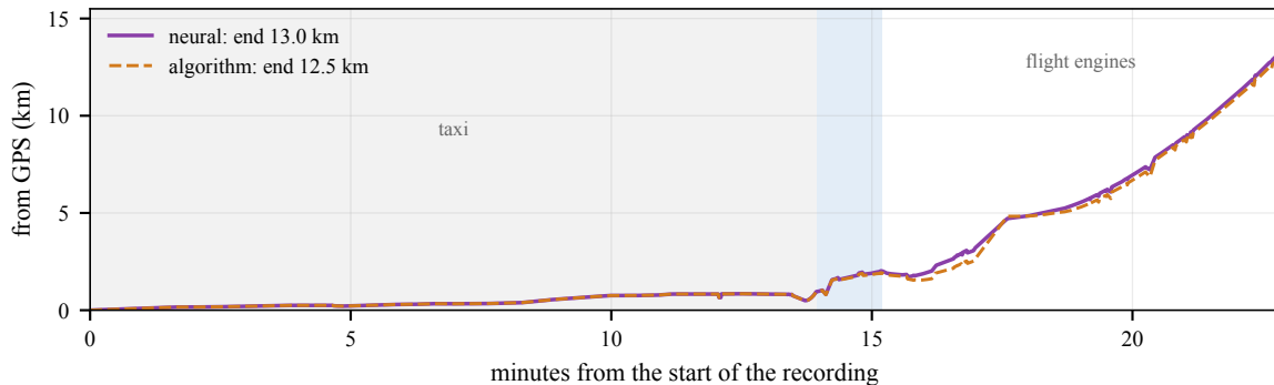
(b) How far the drawn position is from GPS
