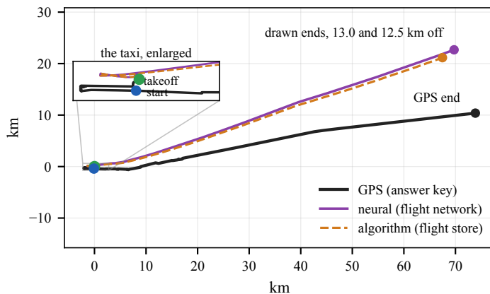
(a) The whole flight drawn from the first GPS point, turned by an arbitrary angle
