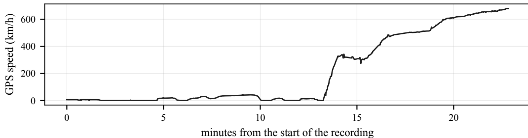
(b) Speed, for the phases of the flight
