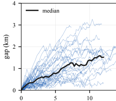
(f) Car: gap, 28 routes
