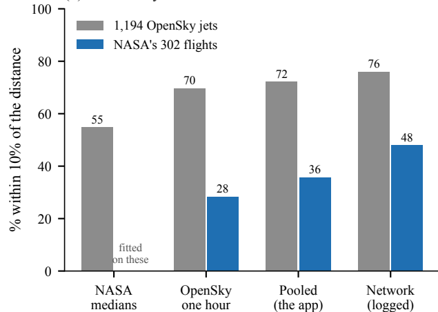
(d) Held out by aircraft
