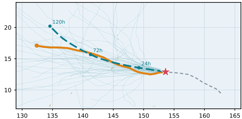
Bavi (2026) — well-behaved recurver 120 h error: 415 km (v8 448, improved)
