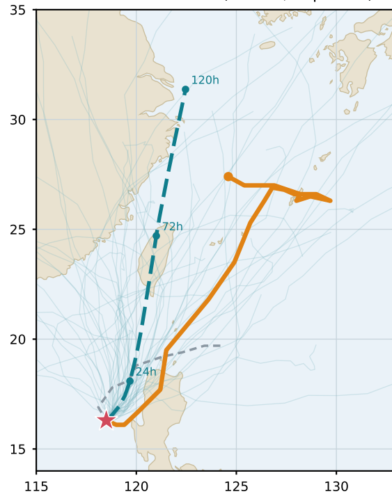
Co-may (2025) — erratic recurvature 120 h error: 488 km (v8 949, improved)
