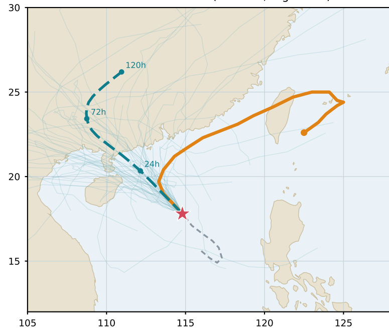
Wayne (1986) — five loops 120 h error: 1236 km (v8 1024, regressed)
