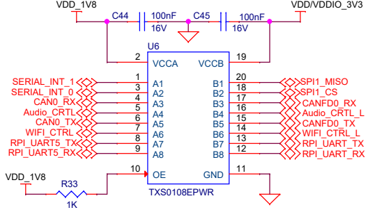
Level Translator for RPI Interface
