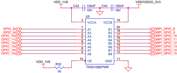
Level Translator for RPI Interface
