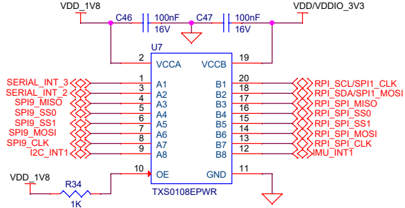
Level Translator for RPI Interface
