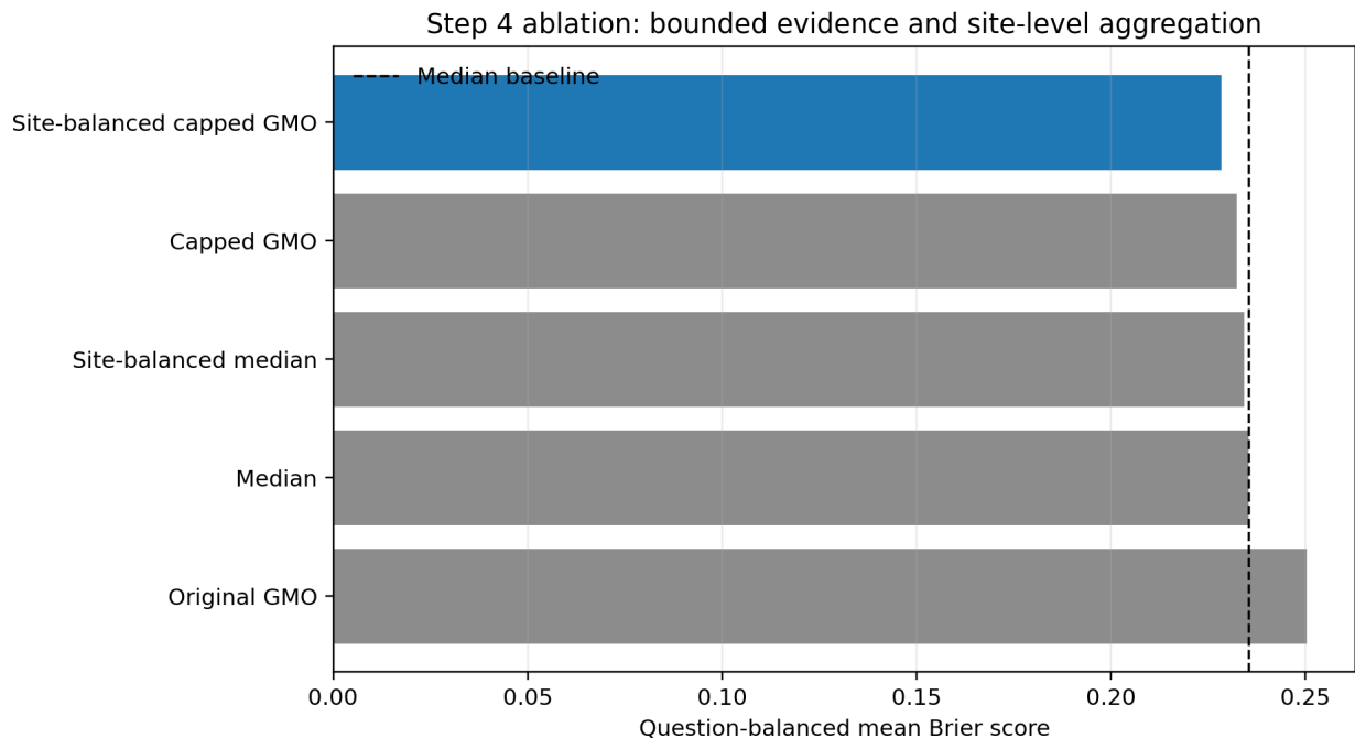
Figure 2: Step 4 ablation
