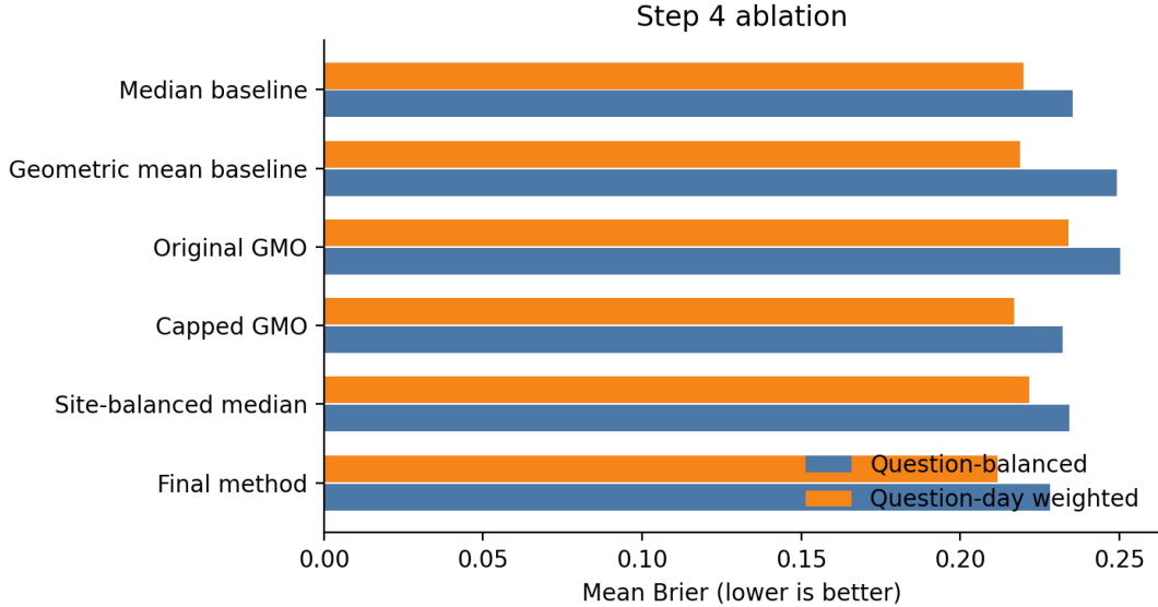
Figure 2: Step 4 ablation
