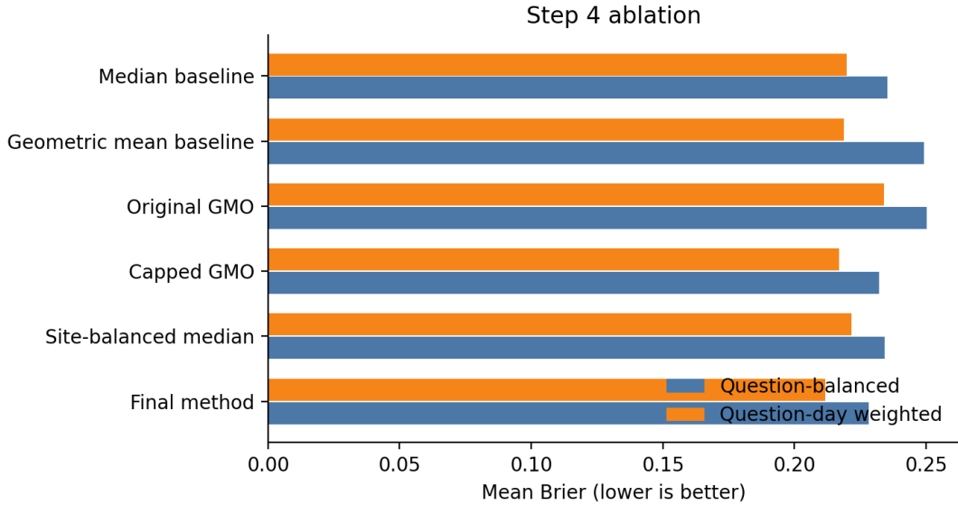
Figure 2: Step 4 ablation
