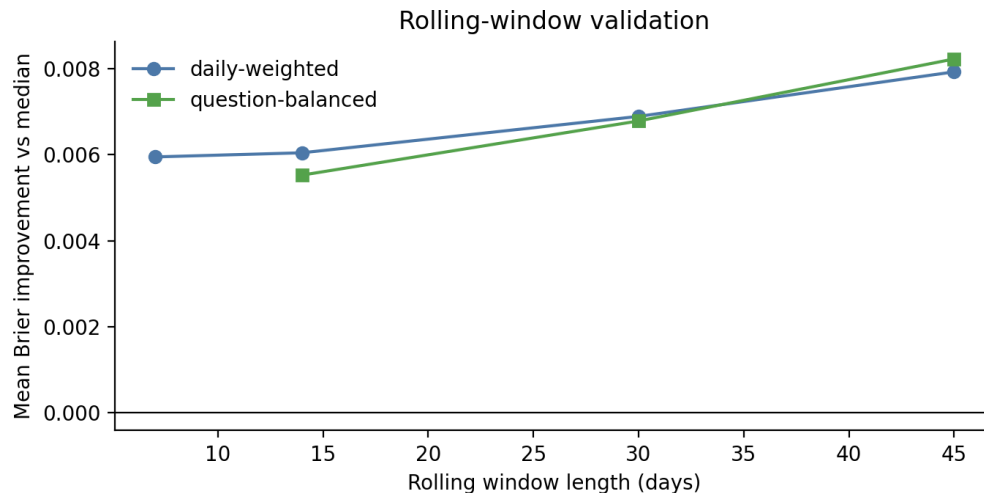
Figure 3: Rolling-window validation
