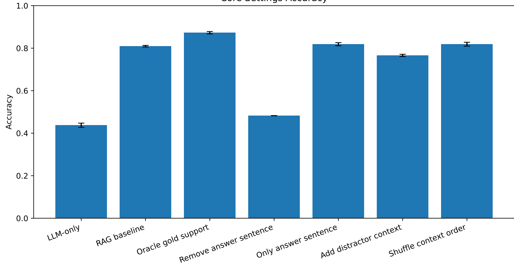
Core Settings Accuracy
