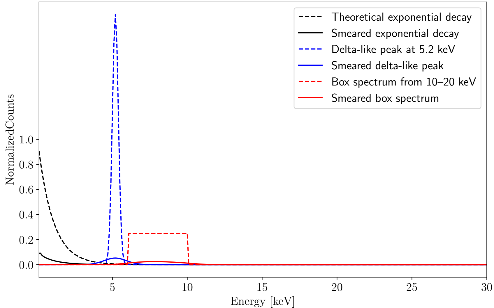
XENON1T Spectrum with Energy Resolution Smearing
