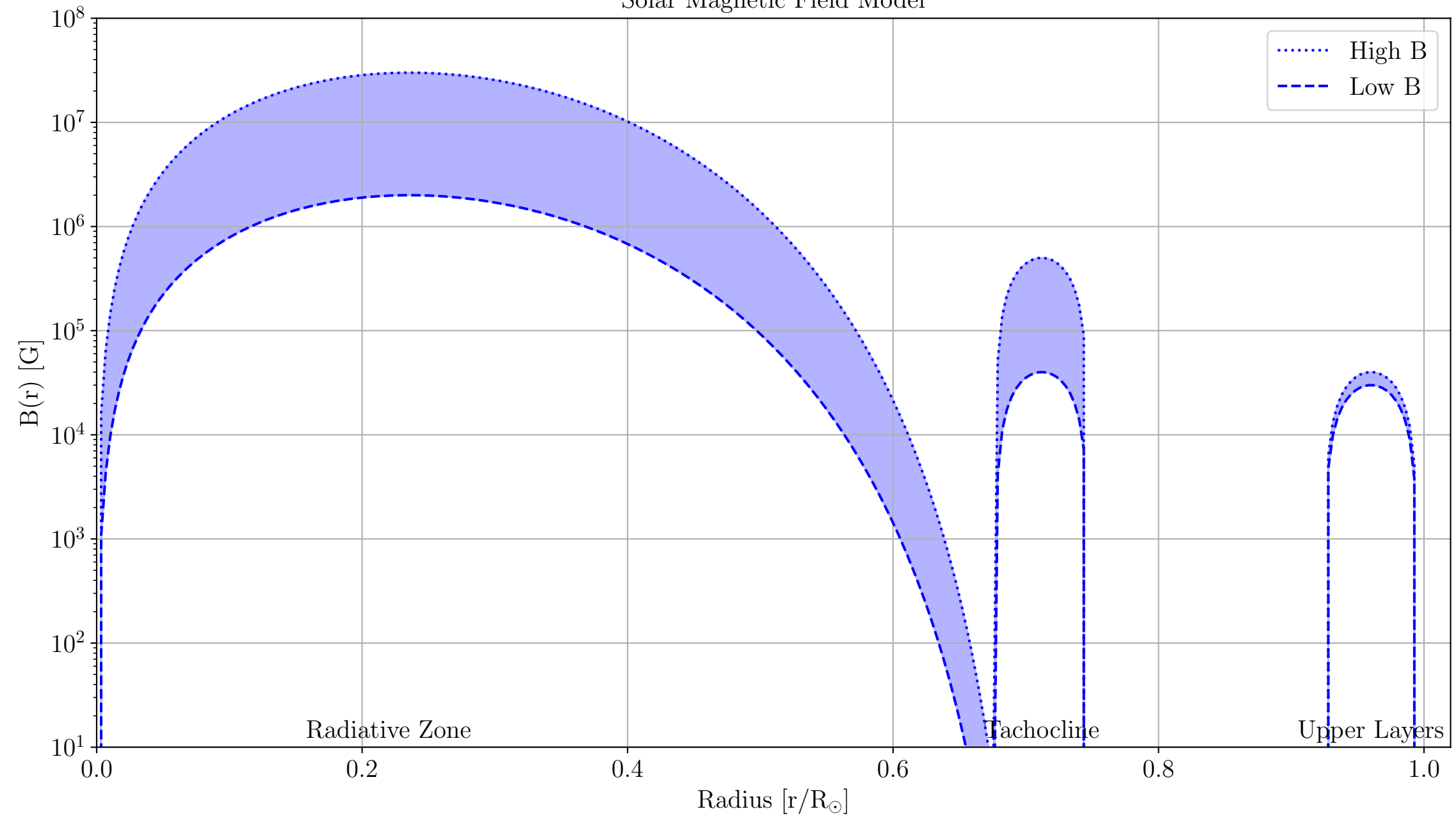
Solar Magnetic Field Model
