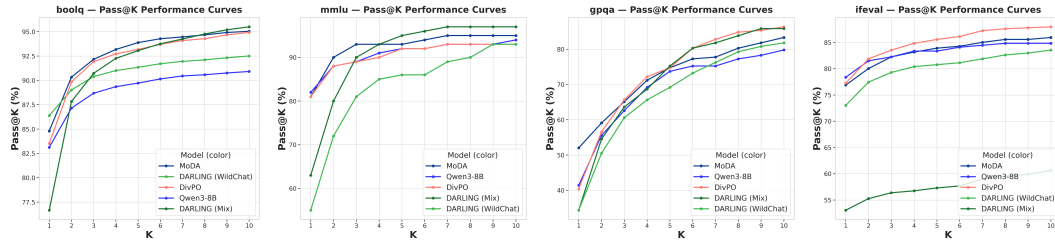
Figure 7: General capability retention: pass@k accuracy. Qwen3-8B base and thinking disabled models on the general capability suite tasks: BoolQ, MMLU, GPQA, and IFEval.
