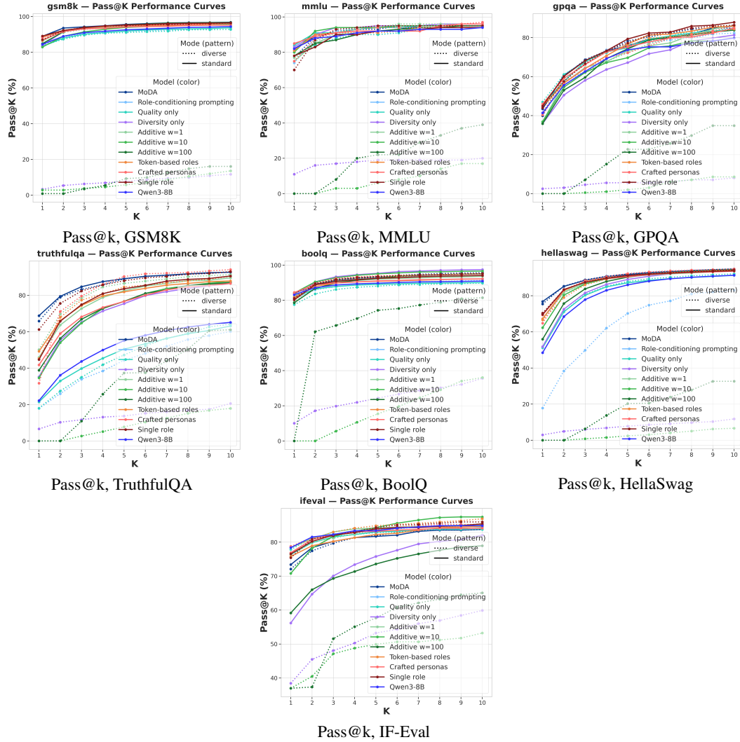
Figure 11: General capability retention for ablated models: pass@k accuracy by benchmarks, standard vs diverse decoding mode.
