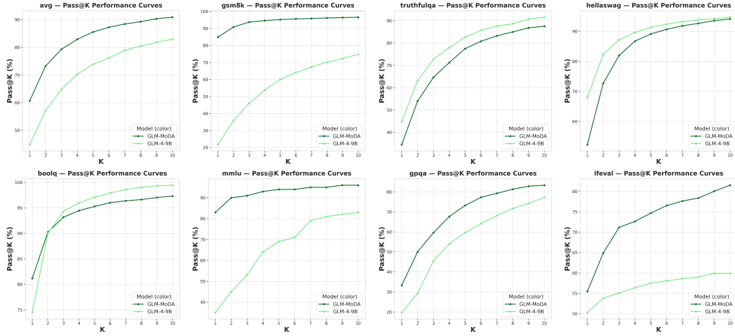
Figure 10: General capability retention: pass@k accuracy. GLM-4-9B base and thinking disabled models.
