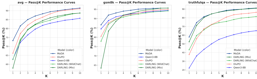
Figure 4: General capability retention: pass@k accuracy. Qwen3-8B base, thinking disabled models on the general capability suite average, GSM8K and TruthfulQA. More results can be found in Appendix B.2 Figure 4.
