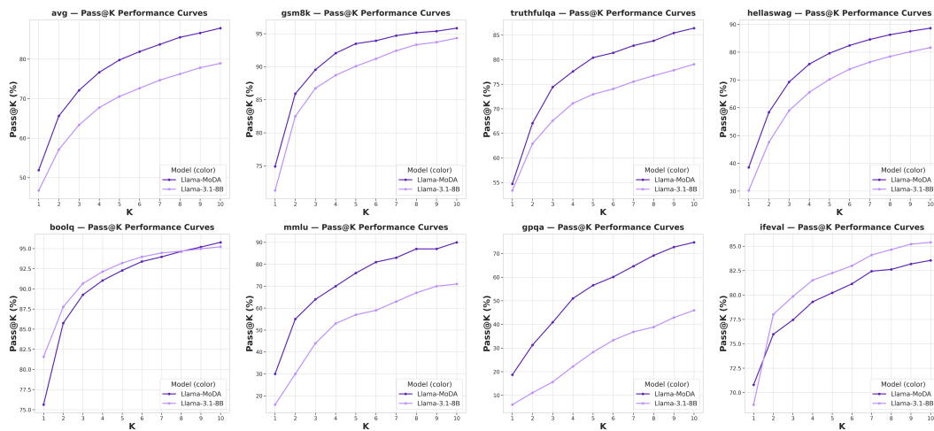
Figure 9: General capability retention: pass@k accuracy. Llama-3.1-8B base and thinking disabled models.
