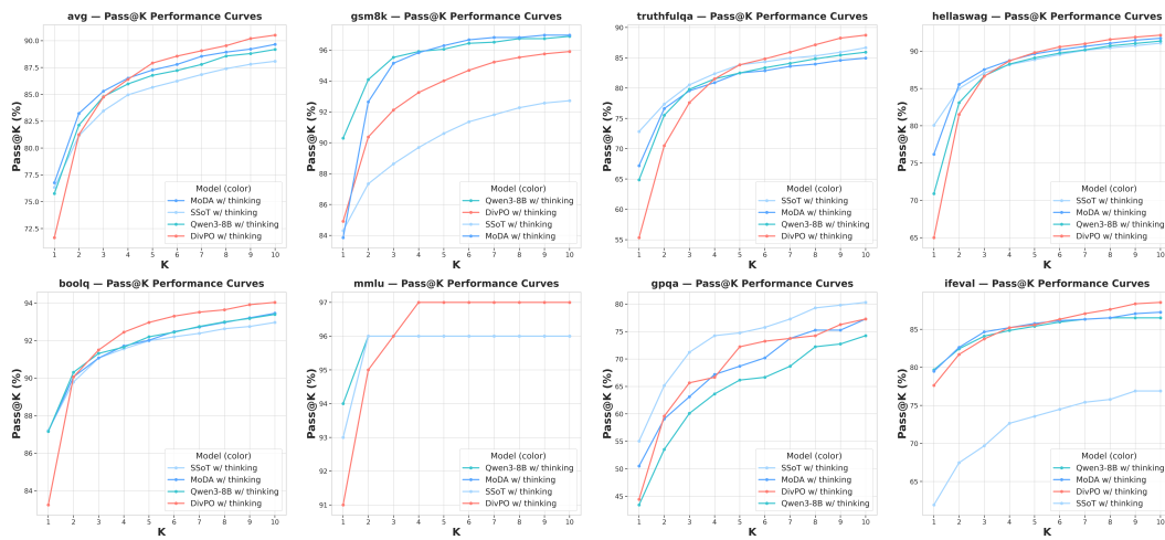
Figure 8: General capability retention: pass@k accuracy. Qwen3-8B base and thinking enabled models.
