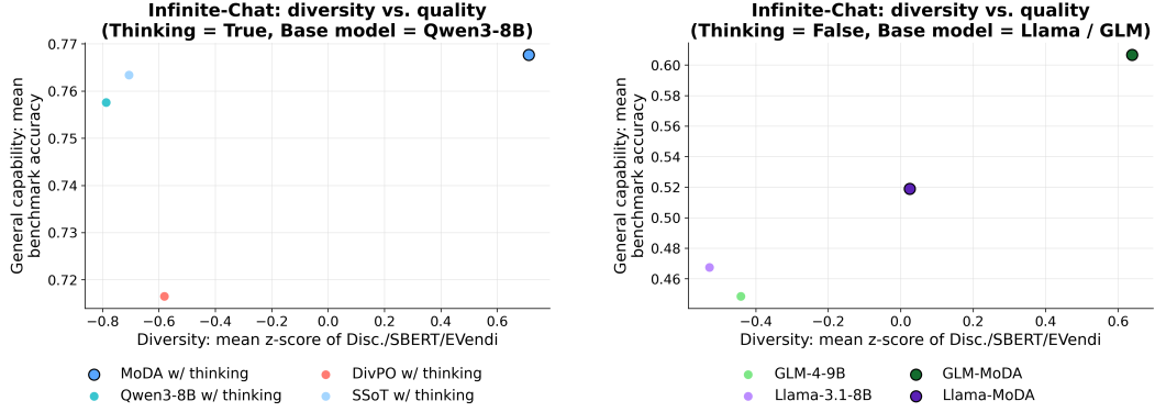
Figure 7: Diversity vs. quality pareto fronts, remaining settings (extends Figure 2 in the main text). The x-axis is Infinite-Chat response diversity (mean z-score of Disc./SBERT/EmbVendi) and the y-axis is general capability (mean benchmark accuracy). Left: Qwen3-8B base, thinking enabled. Right: Llama-3.1-8B / GLM-4-9B base, thinking disabled. MoDA Pareto-dominates all baselines in both settings.
