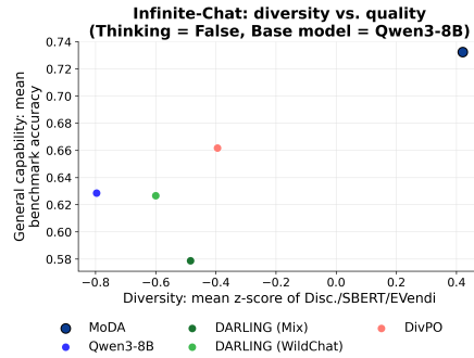
Figure 2: Diversity vs. quality pareto front (Qwen3-8B base, thinking disabled). The x-axis is Infinite-Chat response diversity (mean z-score of Disc./SBERT/EmbVendi) and the y-axis is general capability (mean benchmark accuracy). MODA Pareto-dominates all the baselines, achieving better diversity and quality simultaneously. Results for Qwen3-8B (thinking enabled) and Llama-3.1-8B / GLM-4-9B (thinking disabled) are shown in Appendix E.1.
