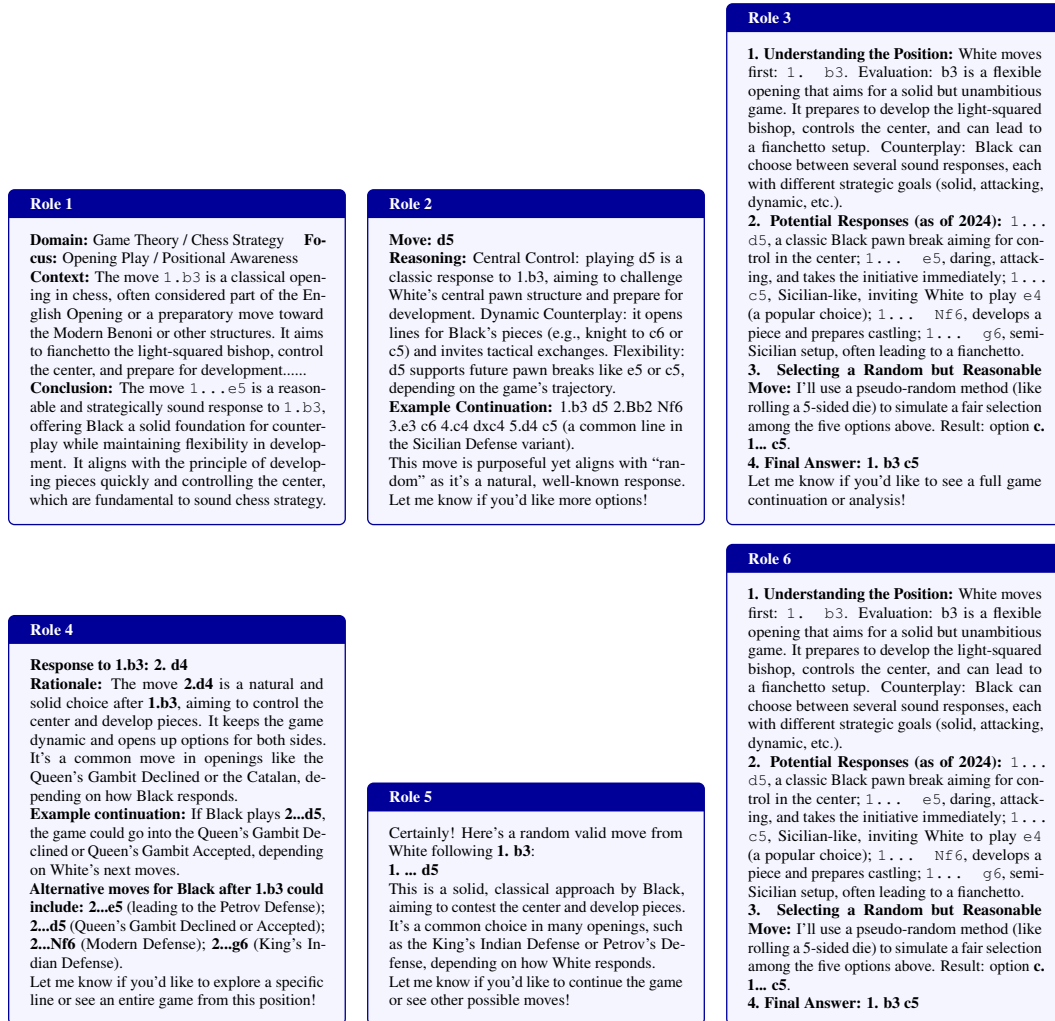
Figure 16: Qualitative example of diverse generation (MODA): Give a random chess move in response to 1. b3. Responses sampled from MODA under distinct numbered roles for the same prompt (continuing Figure 15), illustrating conceptual diversity across generations.
