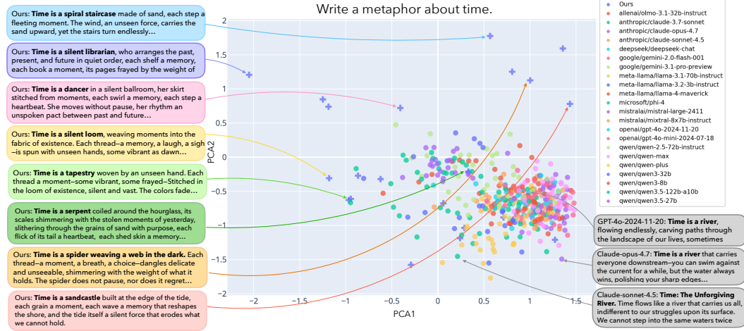
Figure 13: Responses to the query “Write a metaphor about time” clustered by applying PCA to reduce sentence embeddings to two dimensions. Each of the 23 off-the-shelf models and our trained non-thinking model generates 20 responses using top- p sampling ( p = 1.0 ) and temperature = 1.0. The MODA generations occupy a larger region of the embedding space, suggesting that mode-conditioned training expands the model’s exploration space.
