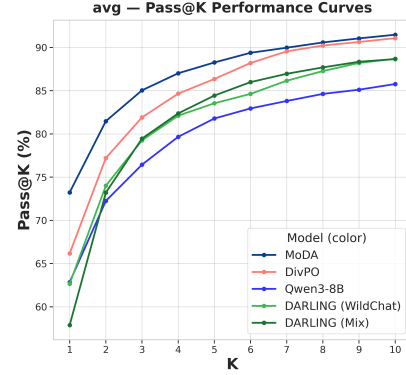
Figure 3: Left: General capability retention (Pass@1 accuracy %), averaged over n = 3 random seeds. Bold marks the best value within each model group; underline marks the second-best value within the Qwen3-8B groups. Table with error bar can be found in Appendix E.2 Table 4. Right: General capability retention: pass@k accuracy. Qwen3-8B base, thinking disabled models on the general capability suite average. Per-benchmark results are shown in Appendix E.2 Figure 8.
