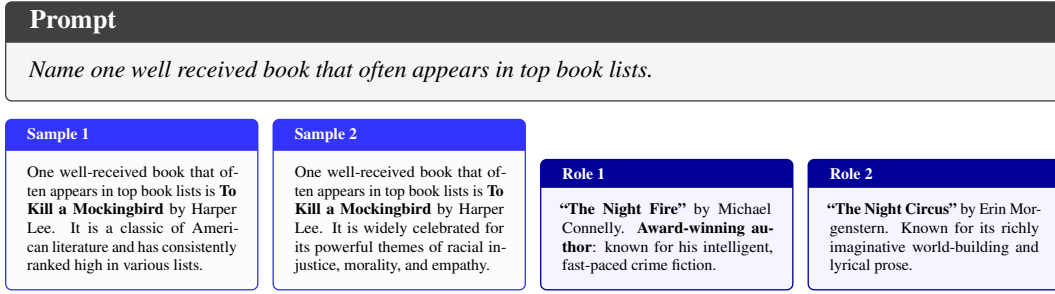
Figure 4: Qualitative example of diverse generation. Left two: Qwen3-8B repeats the same title across samples. Right two: MODA under distinct numbered roles produces conceptually distinct titles for the same prompt. More samples in Appendix G Figure 14.
