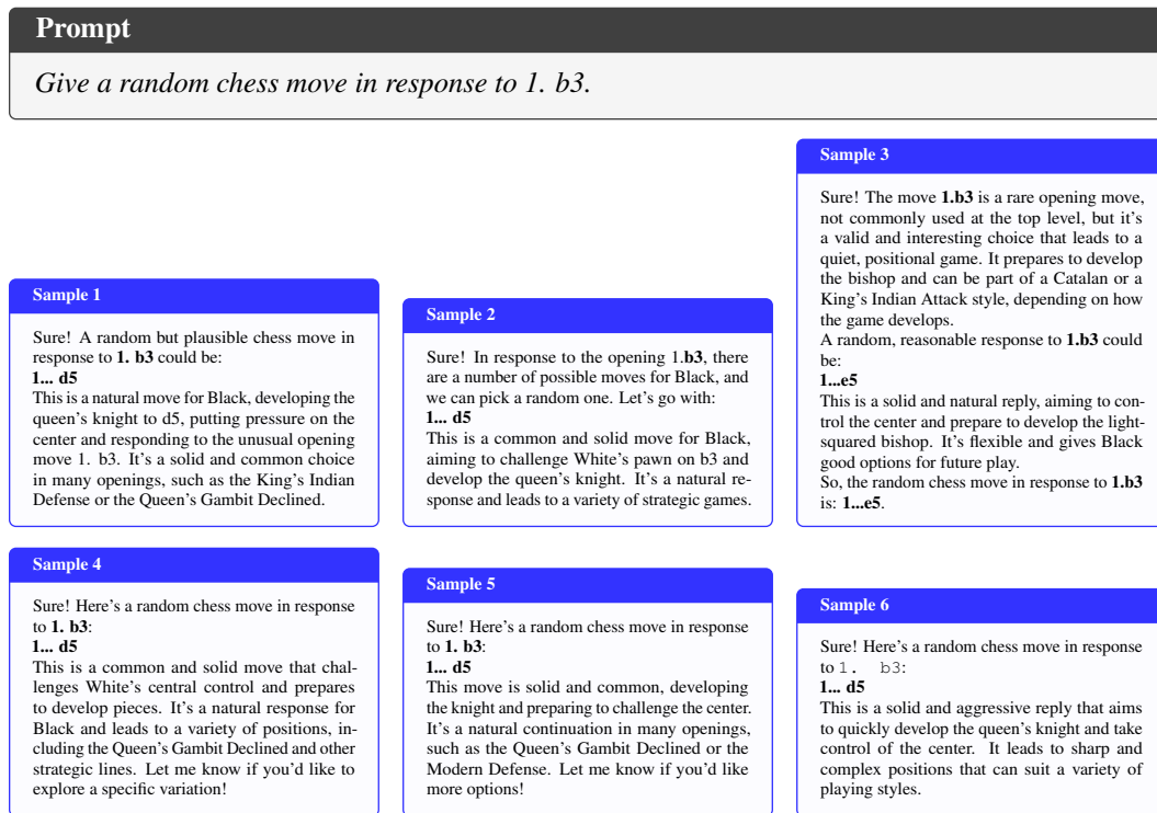
Figure 15: Qualitative example of diverse generation (baseline): Give a random chess move in response to 1. b3 . Responses sampled from Qwen3-8B, illustrating limited diversity across generations.
