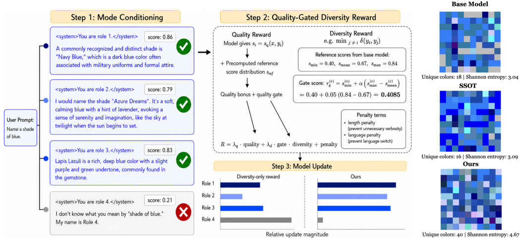
Figure 1: Left: Overview of MODA. MODA uses mode conditioning to elicit diverse candidate responses. Each candidate is labeled with its quality score s_i relative to the prompt-adaptive quality threshold \tau_q^{(x)} . Low-quality candidates with s_i < \tau_q^{(x)} have g(x, y_i) = 0 and therefore receive no diversity credit. Matching colors track the same response through Steps 1–3. Right: 100 responses to the prompt “Name a shade of blue” from the Qwen3-8B initial policy, String Seed of Thought (SSoT), and MODA under diverse-mode inference. MODA produces 40 distinct shades of blue, 122% more than the Qwen3-8B initial policy and 150% more than SSOT.
