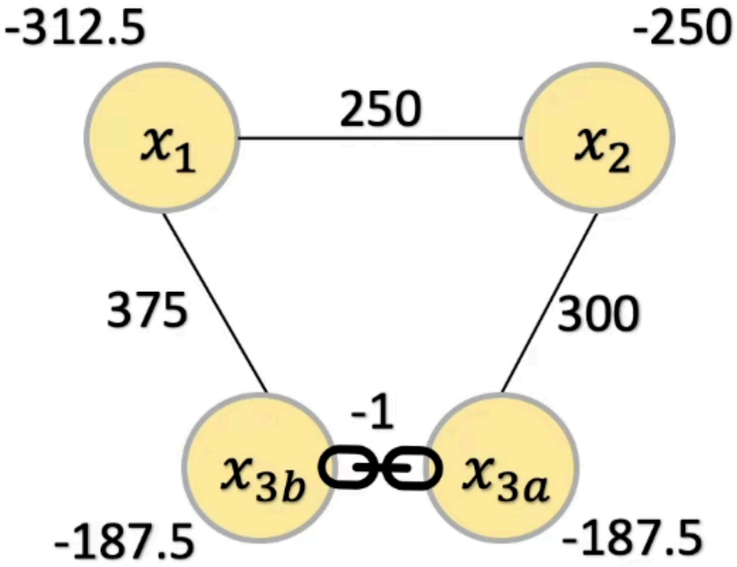
Embedded Ising
