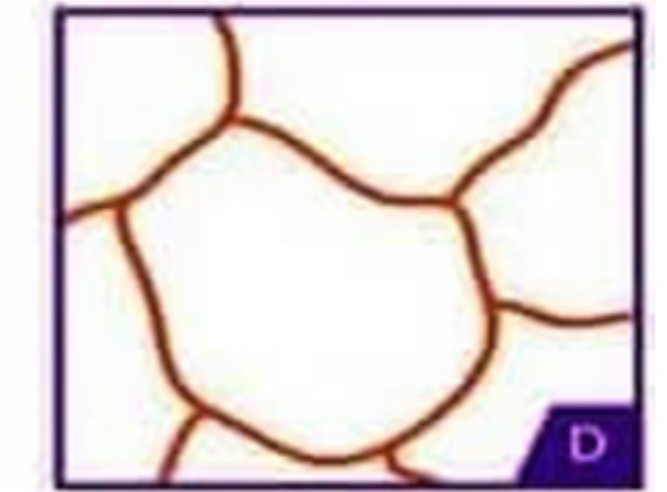
Recrystallization form
