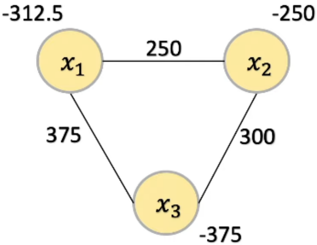
Ising
