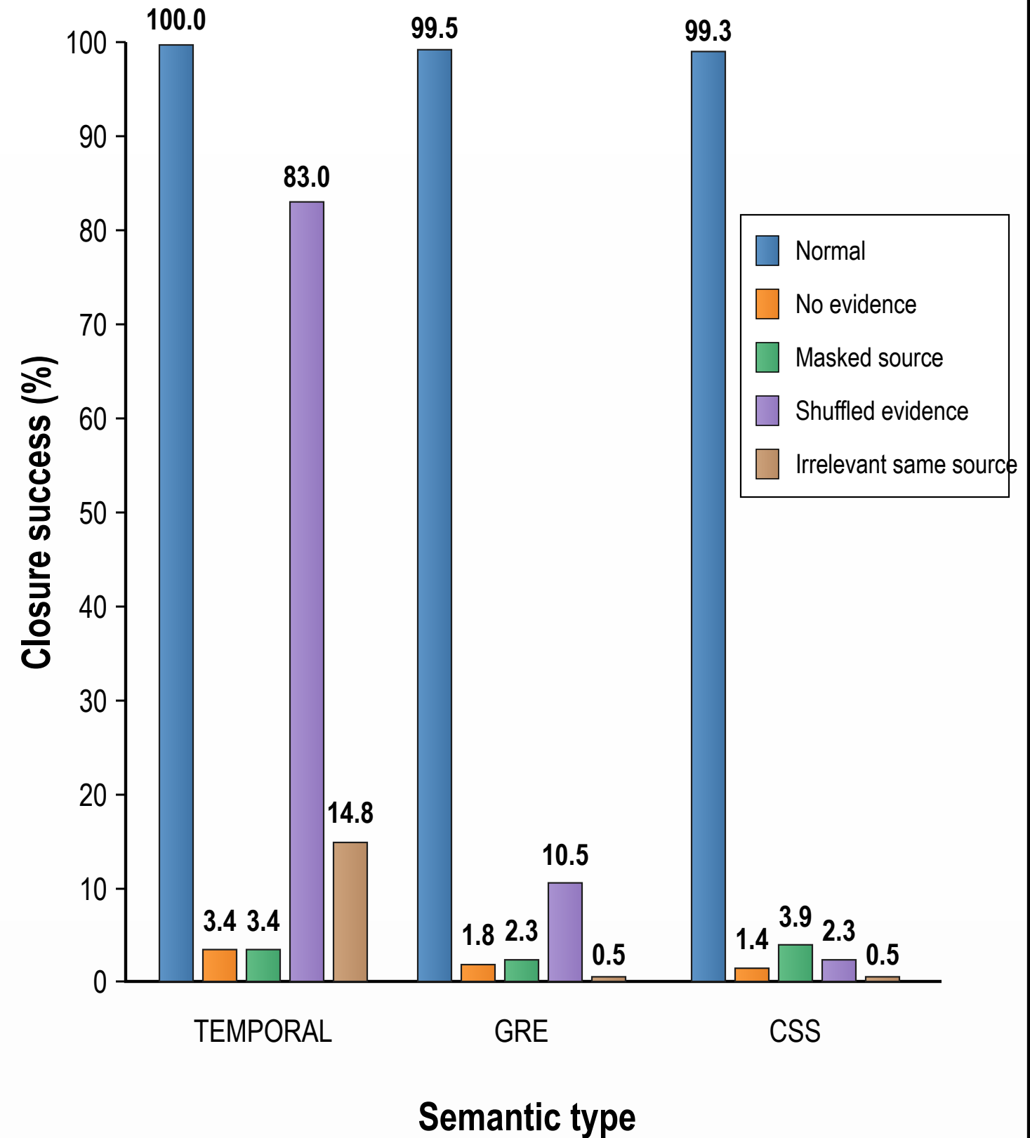
Closure success by semantic type
