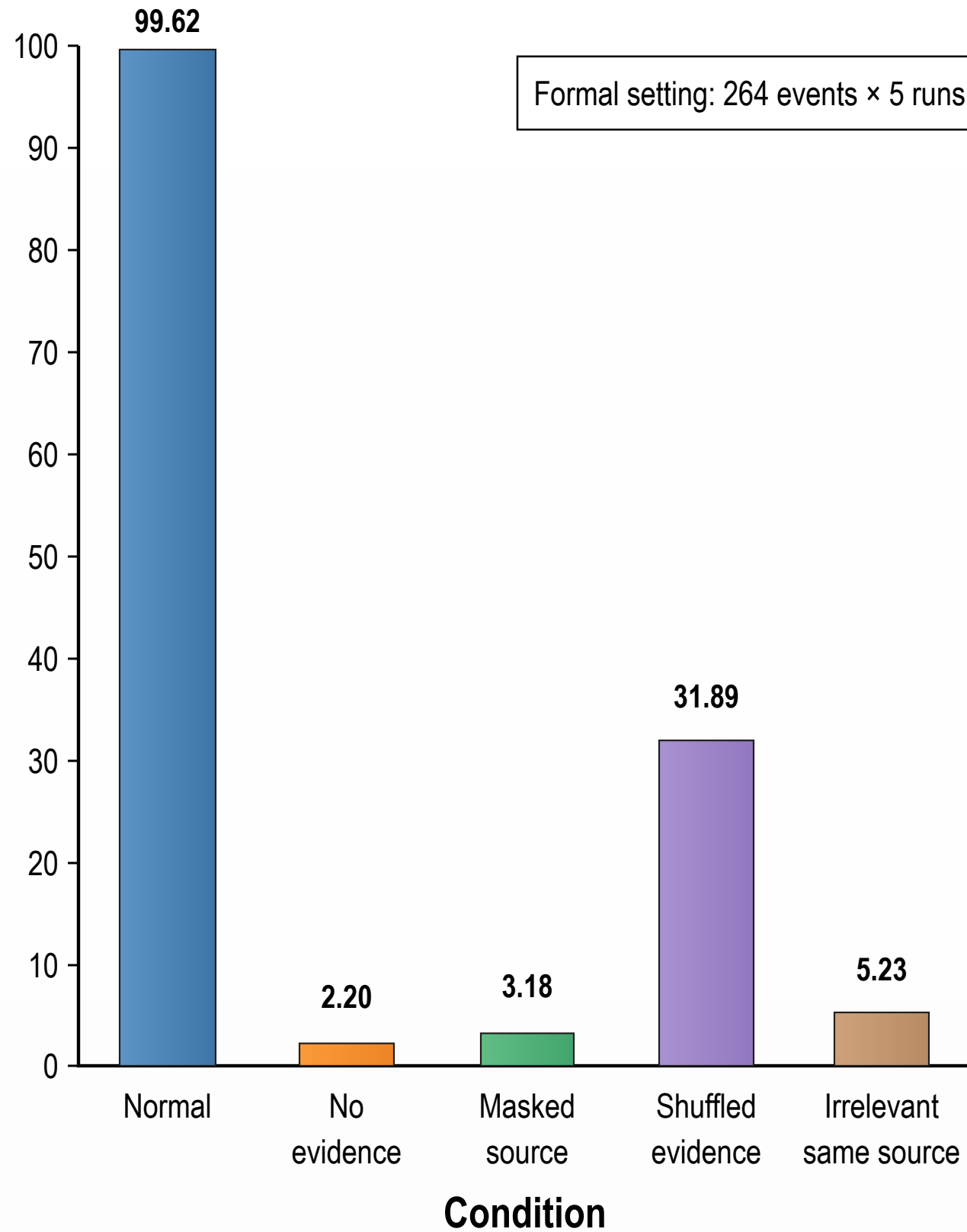
Overall closure success under evidence perturbations
