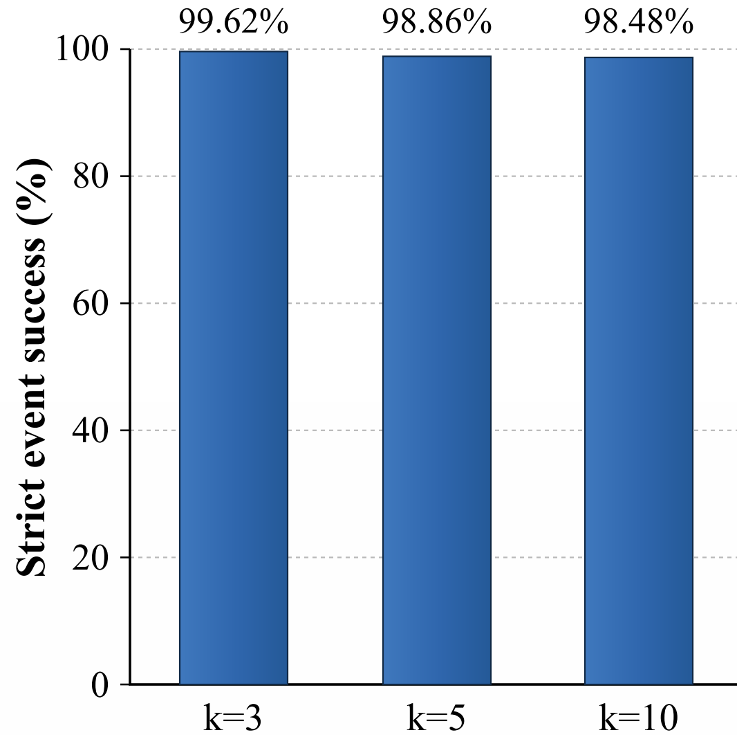
(a) Candidate Pool Size
