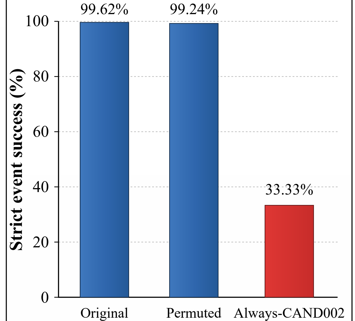
(c) Candidate-Identifier Permutation
