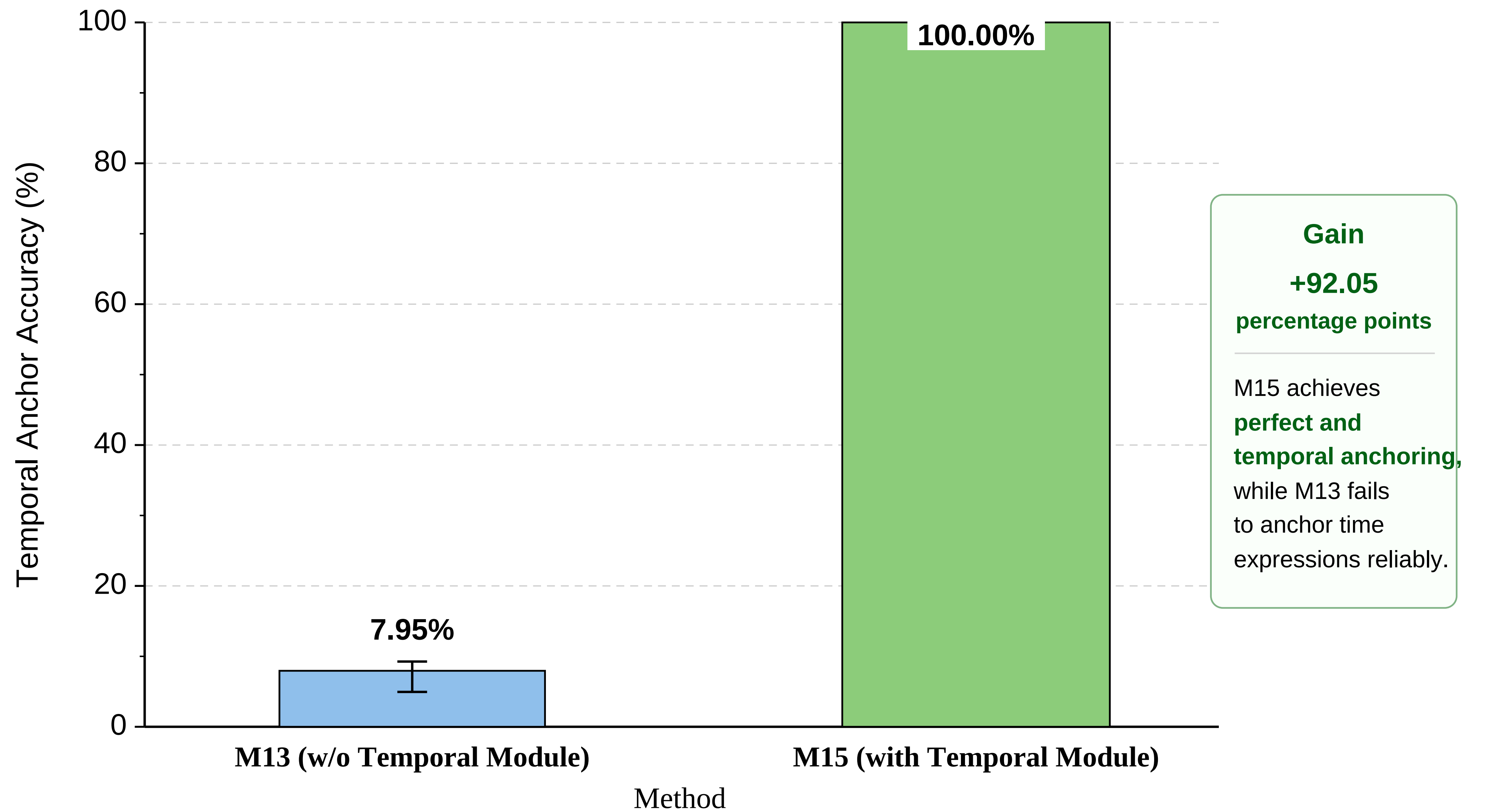
Figure X. Temporal anchor accuracy comparison (Exp13). M13 without temporal modeling fails to resolve temporal context in most cases, while M15 with temporal modeling achieves perfect accuracy.
