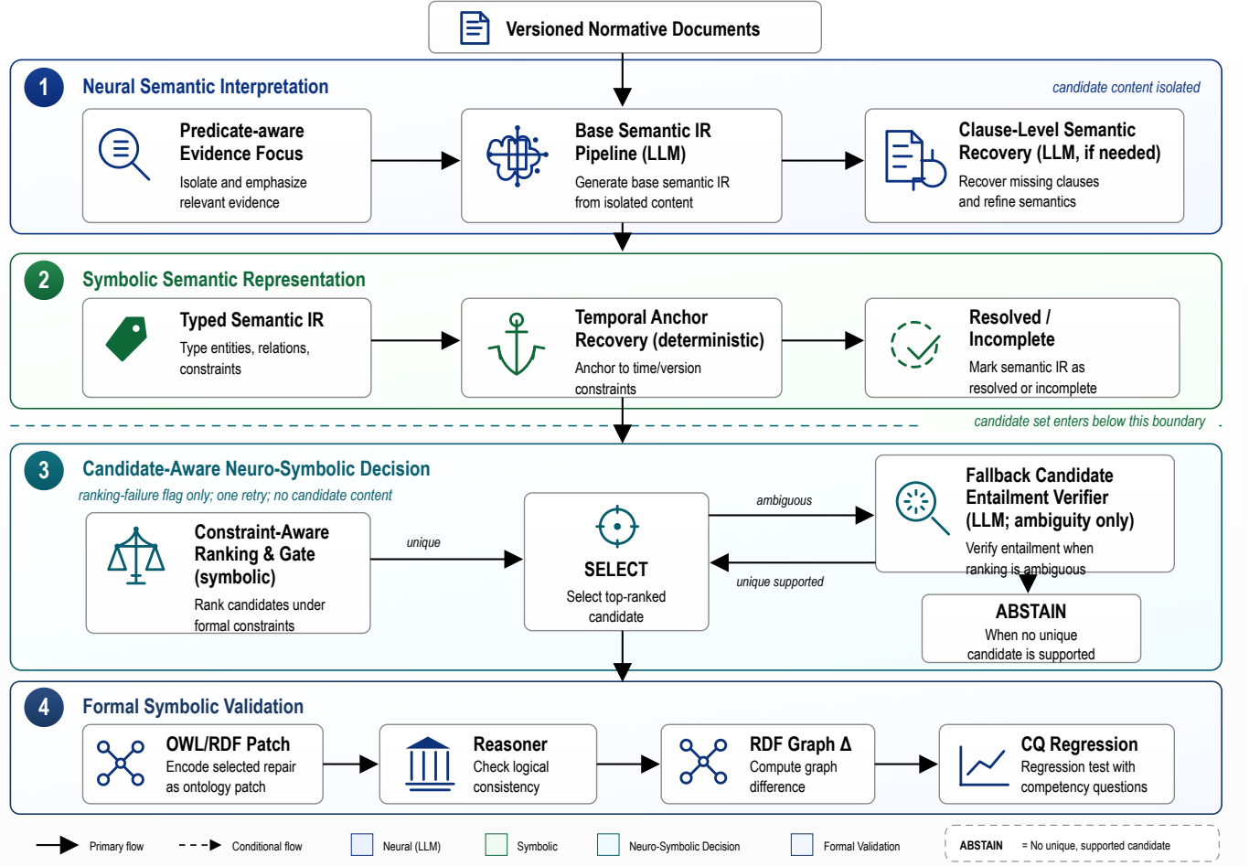
Fig. 1. Overall evidence-constrained neuro-symbolic architecture of ECR-Repair. Semantic IR is the neural-symbolic interface; candidate content becomes visible only after evidence interpretation has been fixed.
