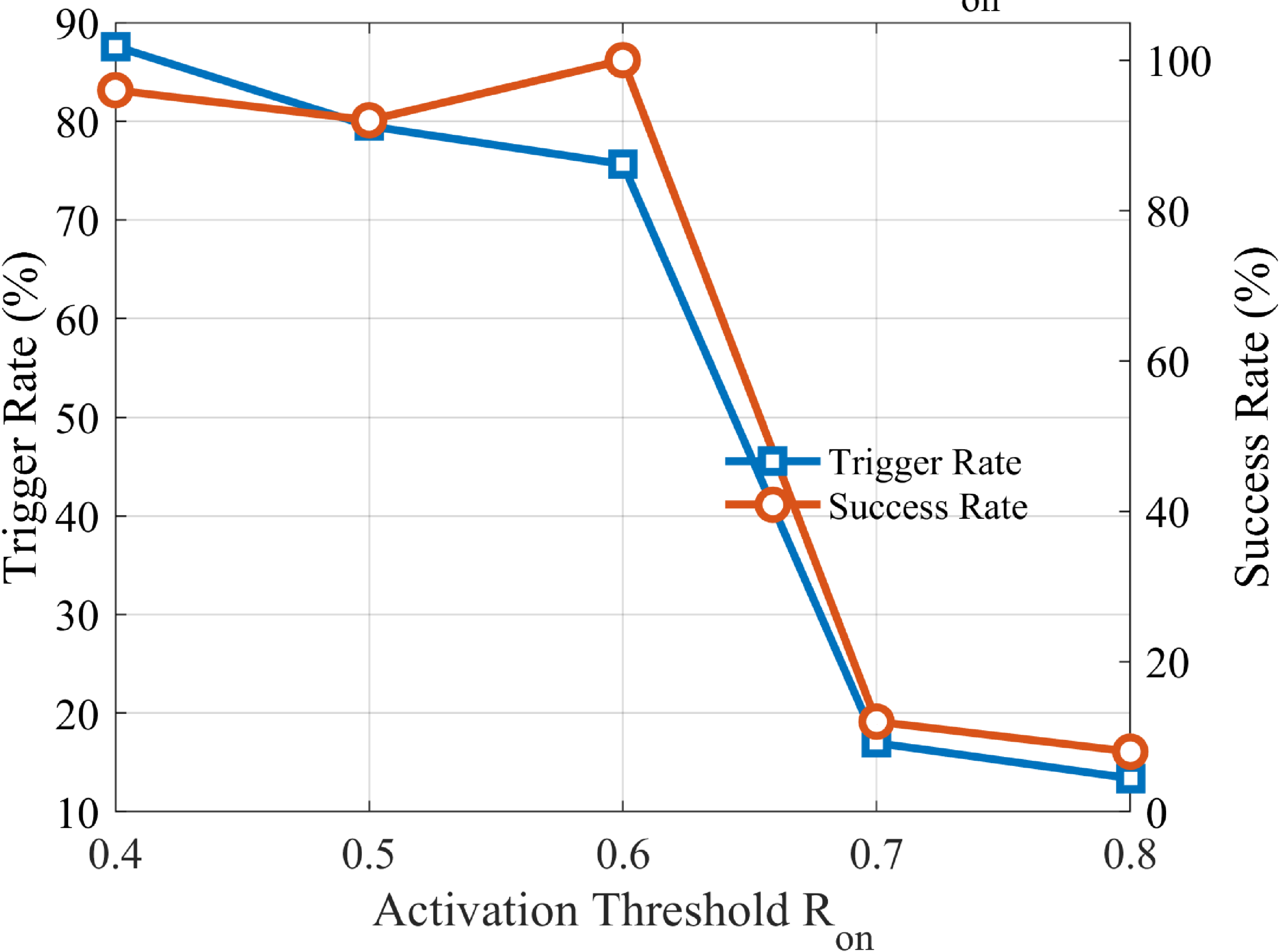
Trigger and Success Sensitivity to R_{on}
