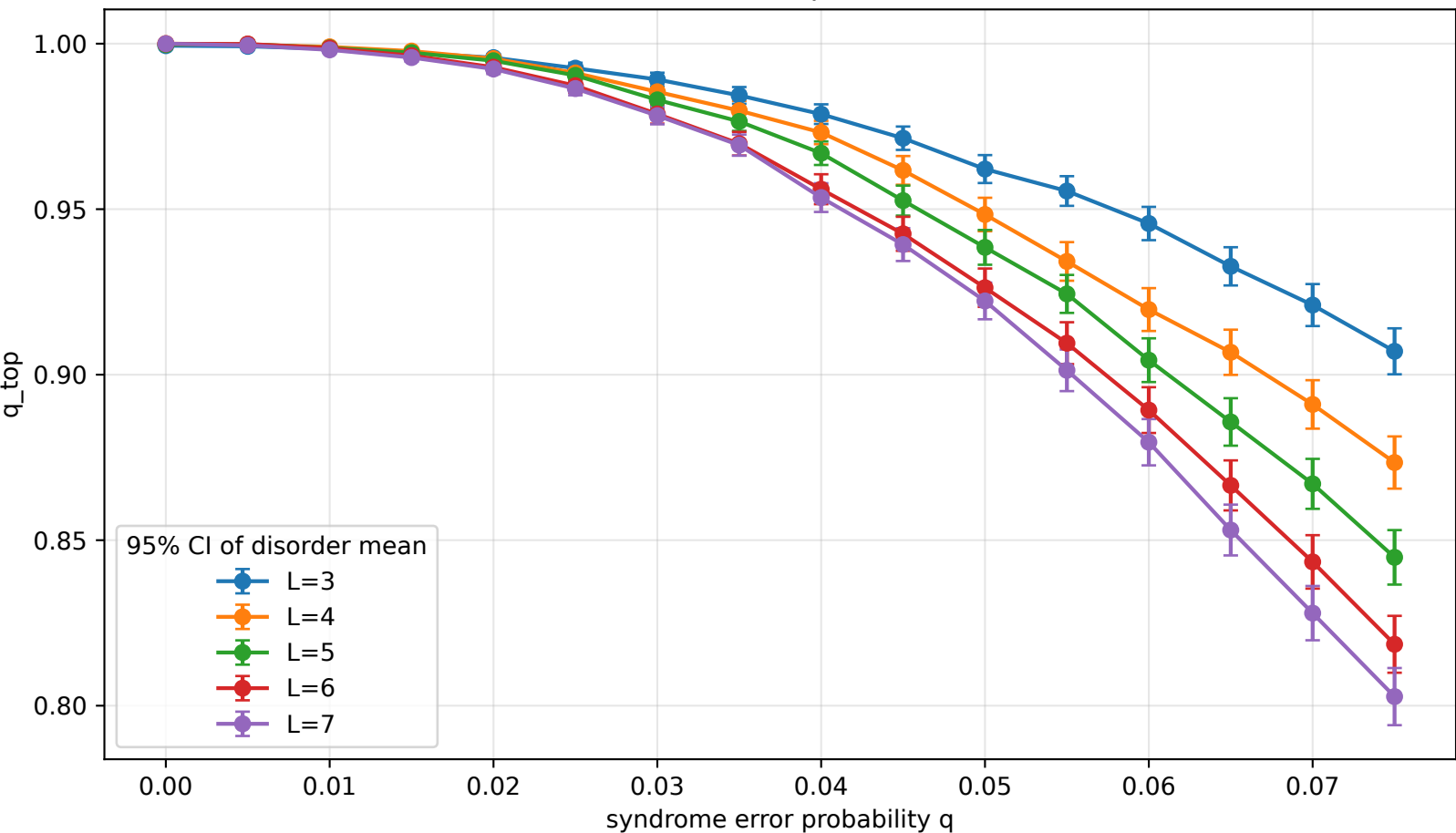
3D toric fixed p=0.0500
