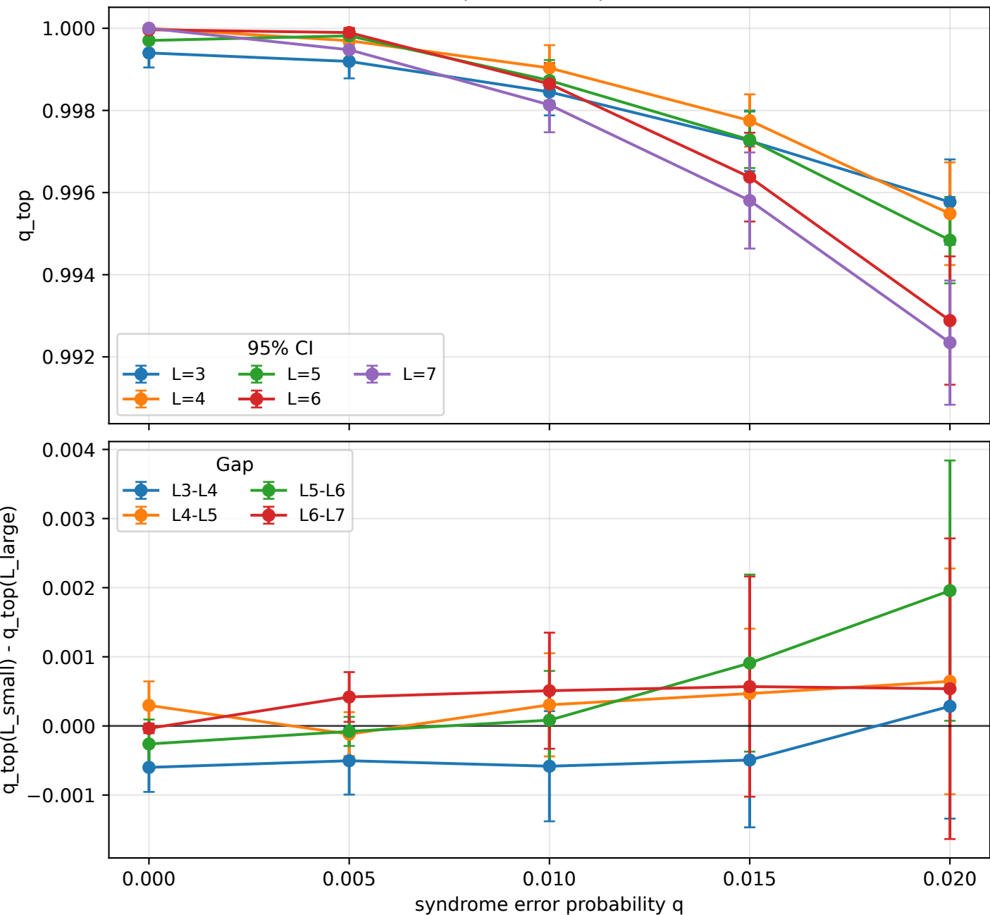
3D toric fixed p=0.0500 , q=0.0000..0.0200
