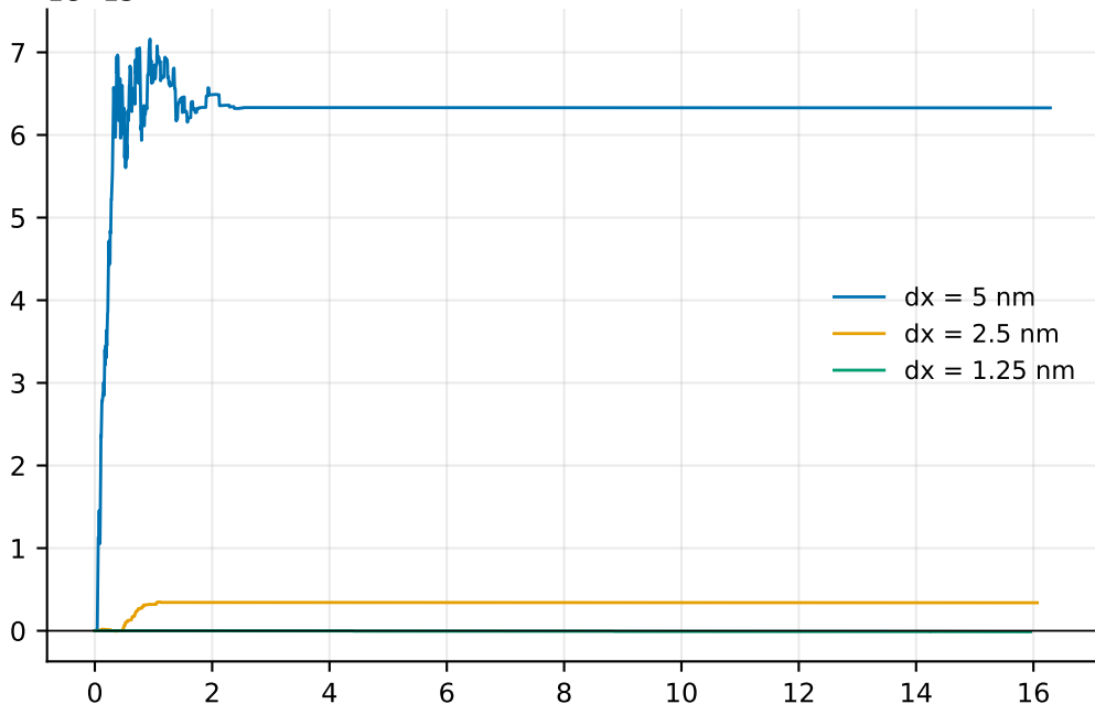
Fluid-mass conservation history
