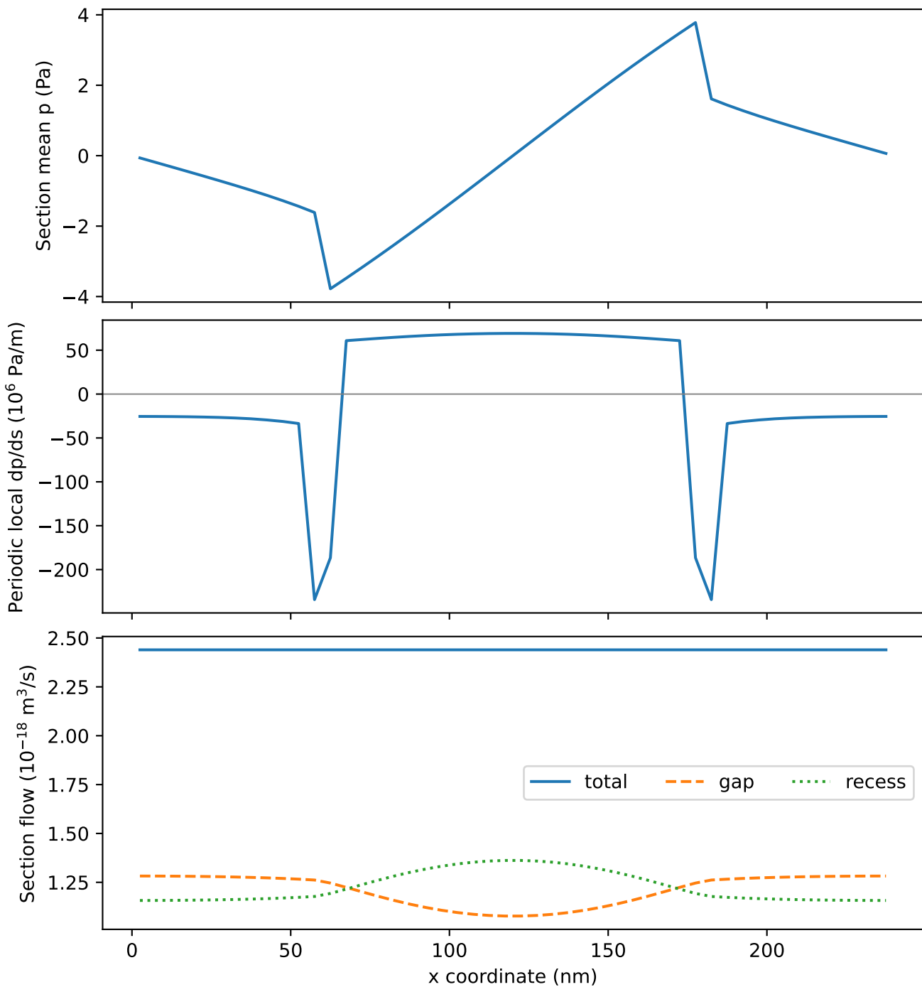
h=65 nm, X drive: pressure and flow distribution
