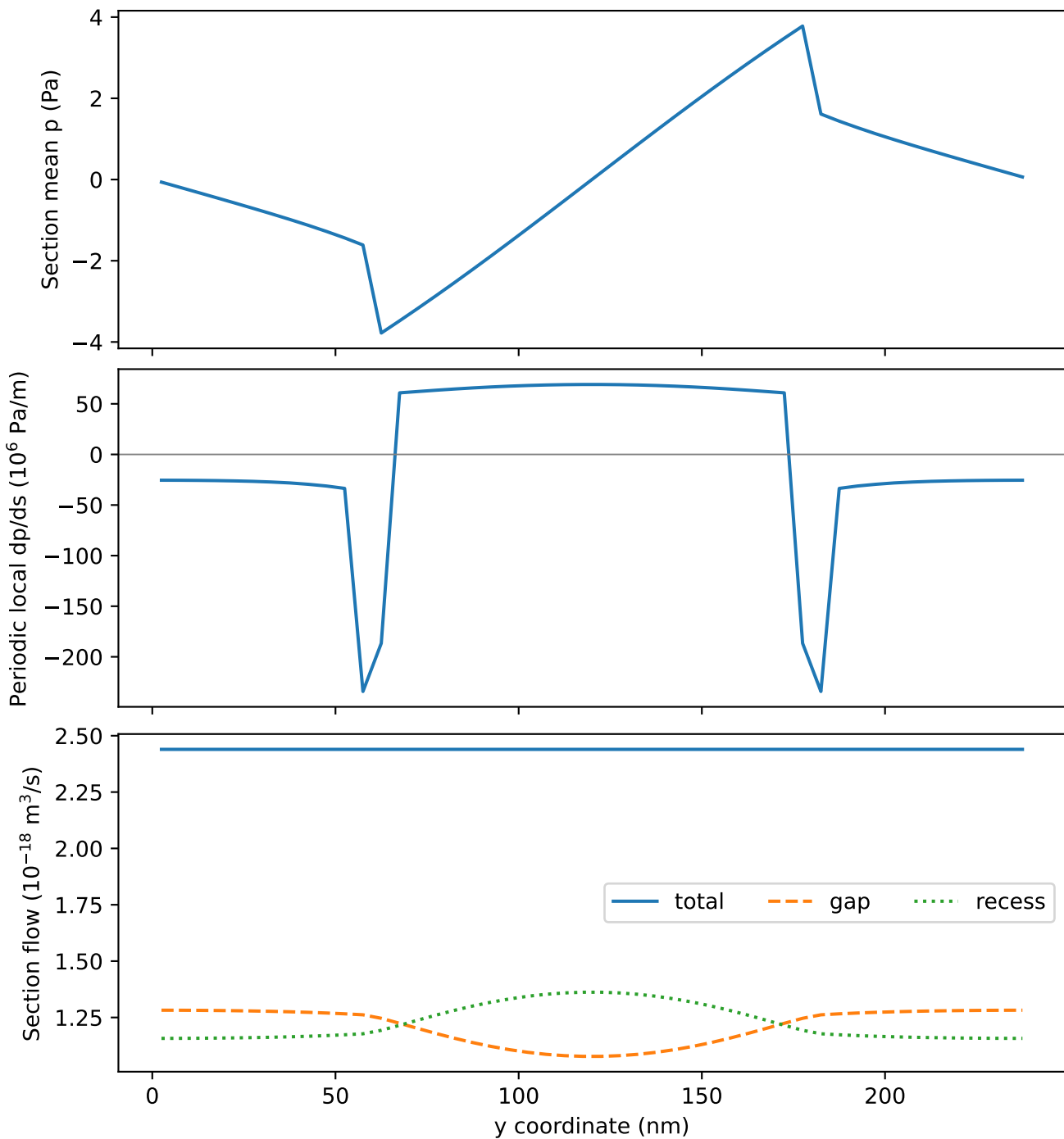
h=65 nm, Y drive: pressure and flow distribution
