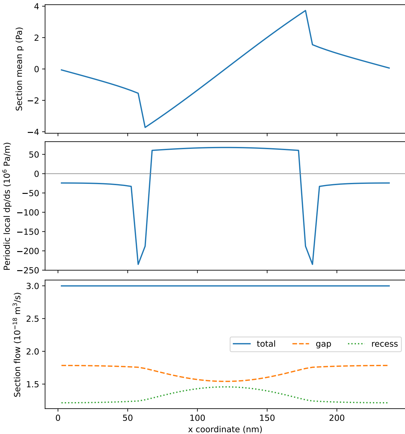
h=75 nm, X drive: pressure and flow distribution
