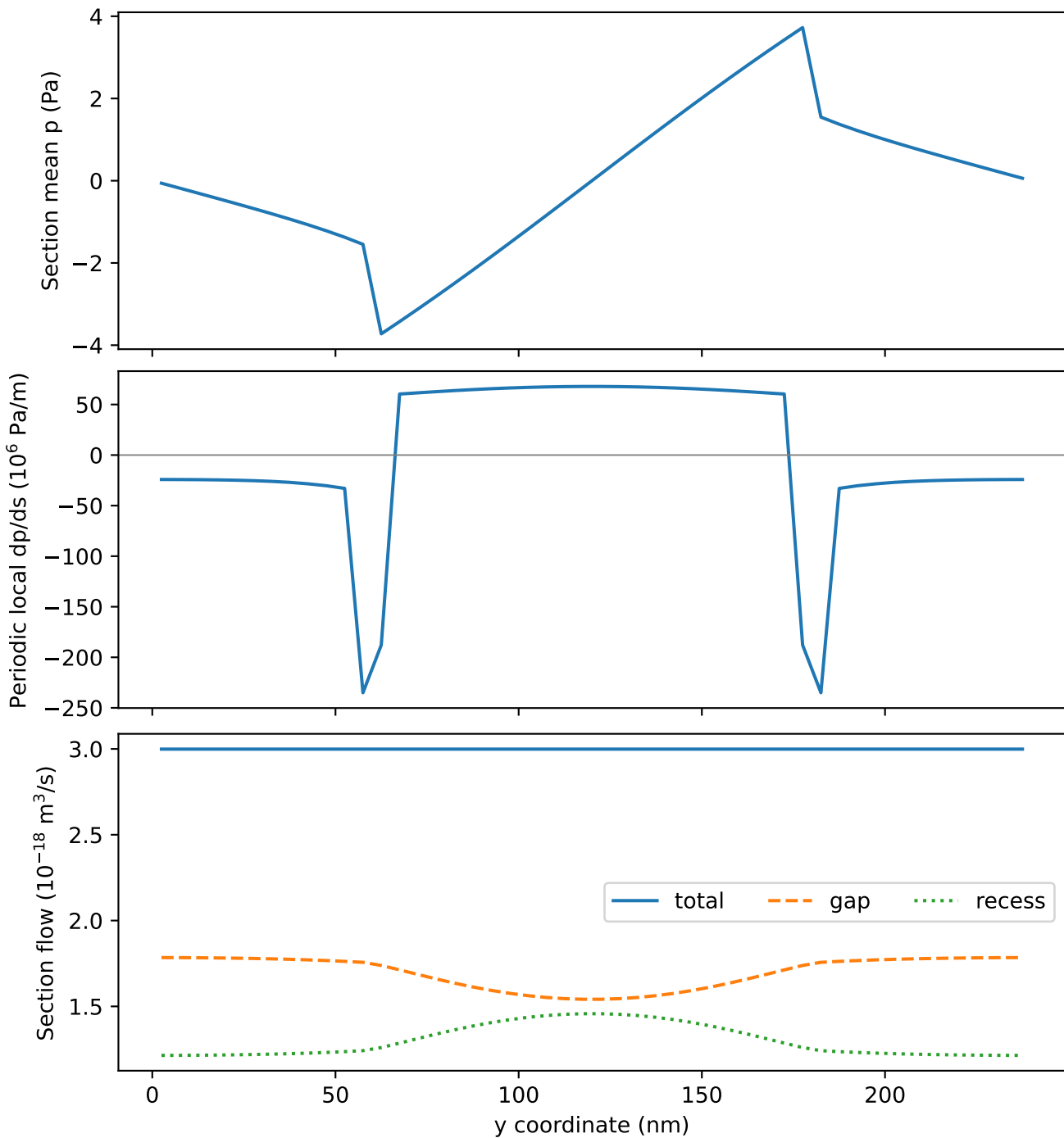
h=75 nm, Y drive: pressure and flow distribution
