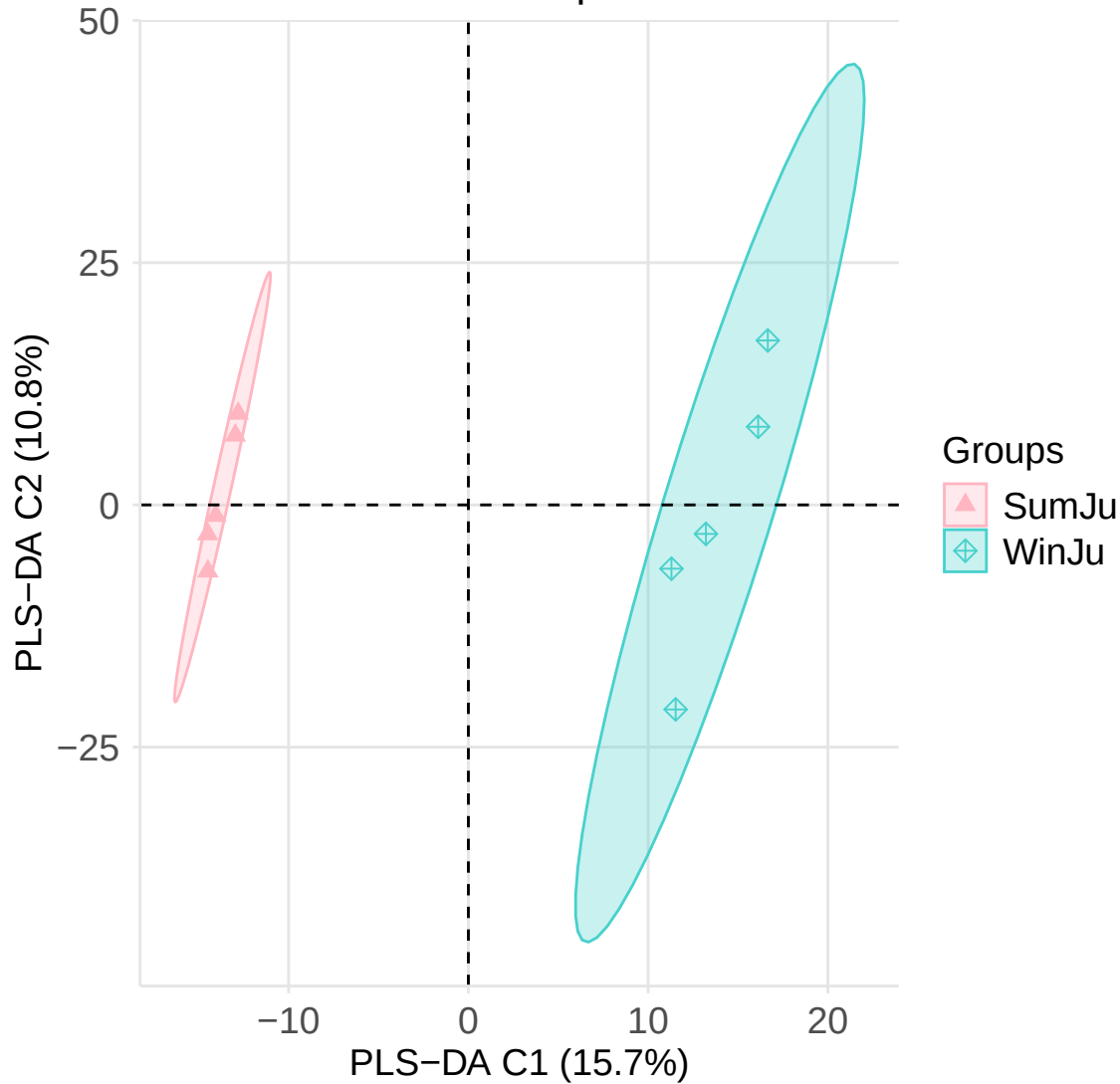
PLS-DA of atrophic Liver
