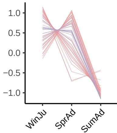
cluster 2 (48)
