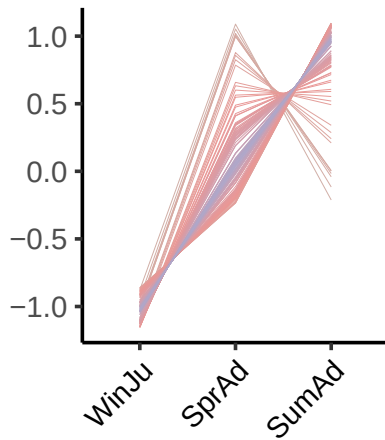
cluster 3 (119)
