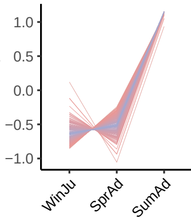
cluster 1 (176)
