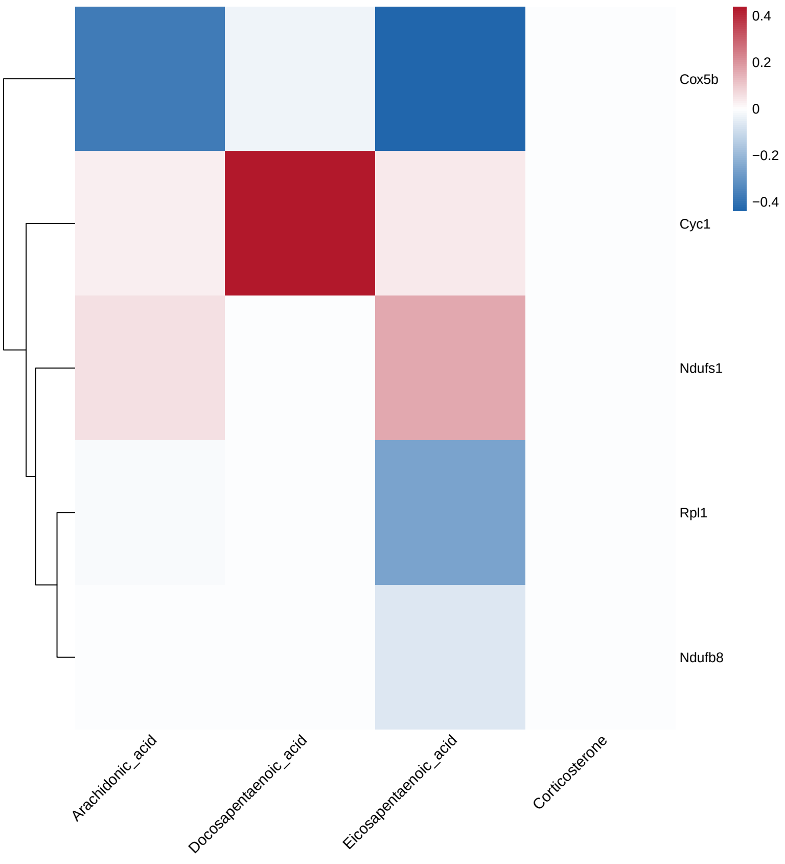
LASSO coefficients Rerown-Liver
