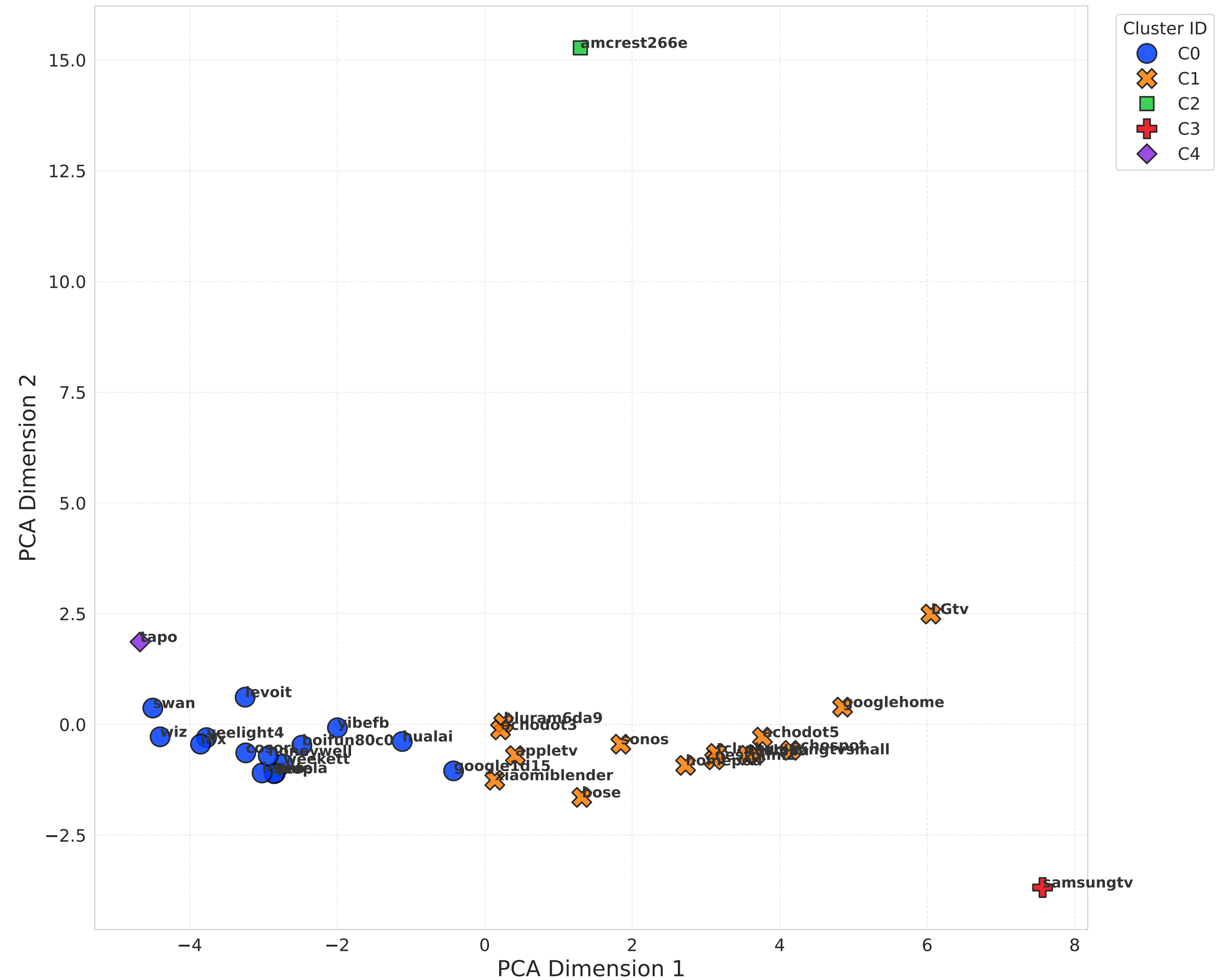
Cluster - PCA Projection
