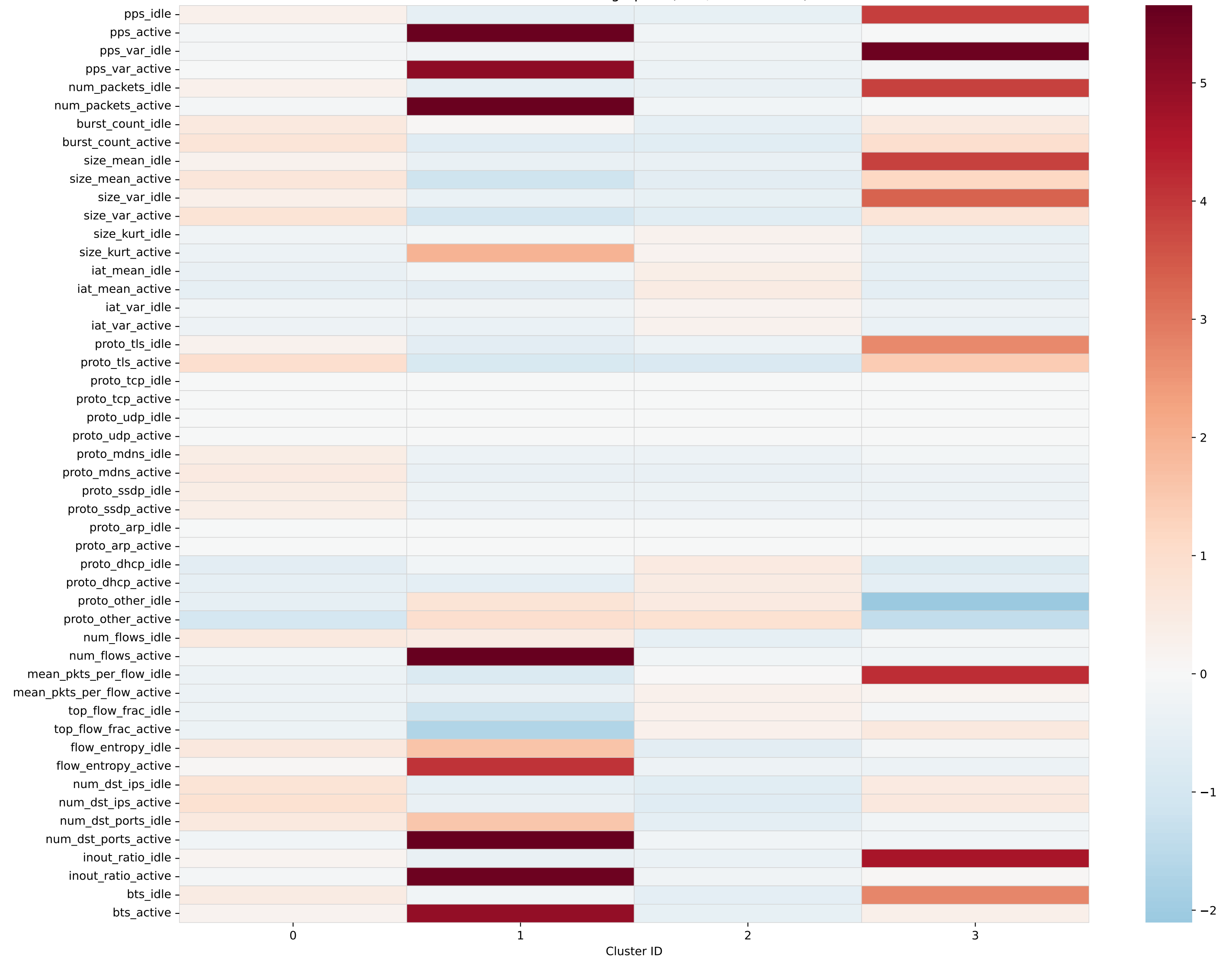
Cluster Behavioral Fingerprint (K=4, Idle + Active)
