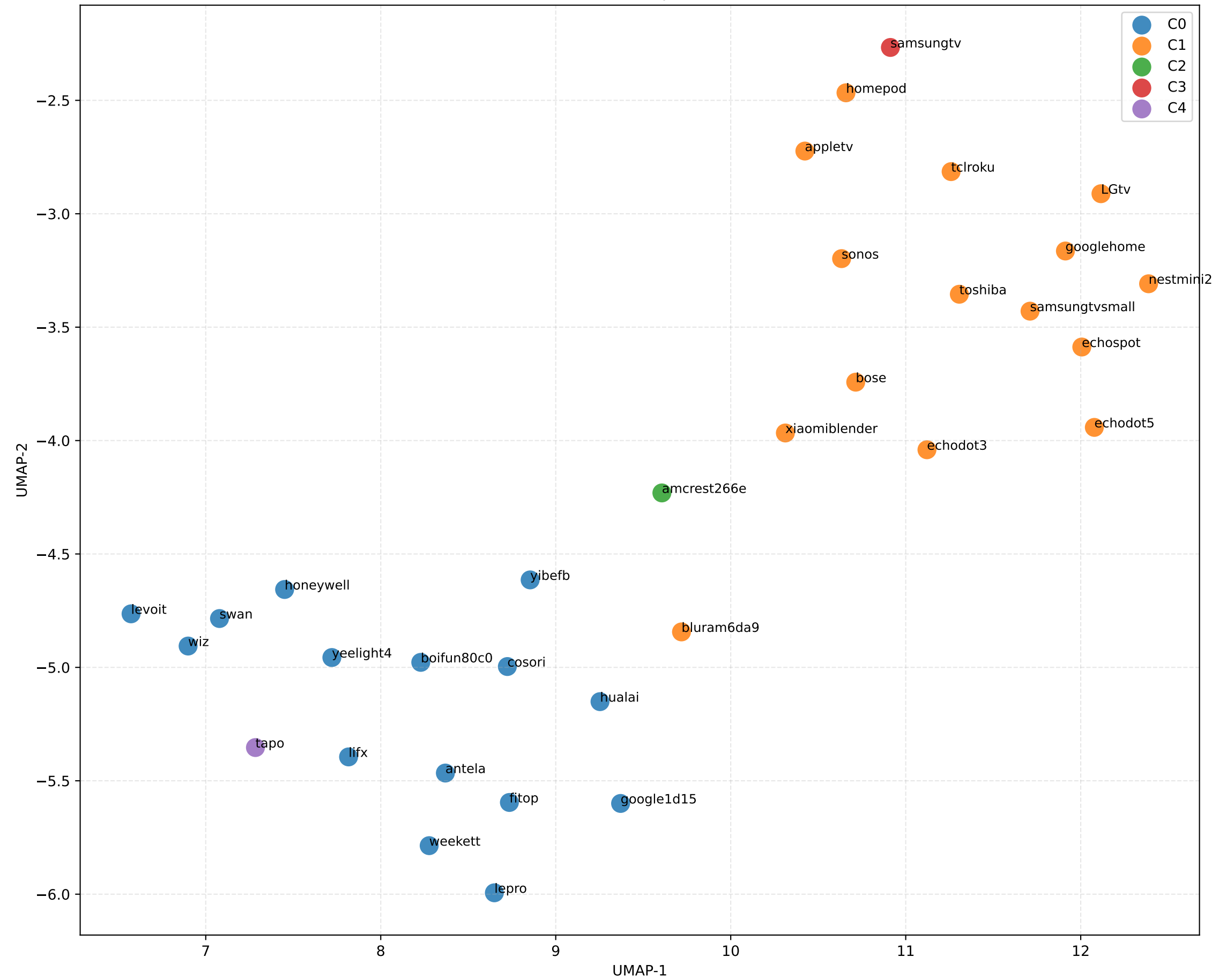
Cluster UMAP Projection (2D)
