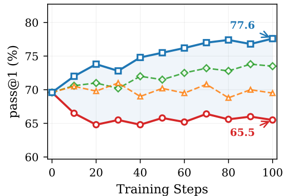
MATH-500
