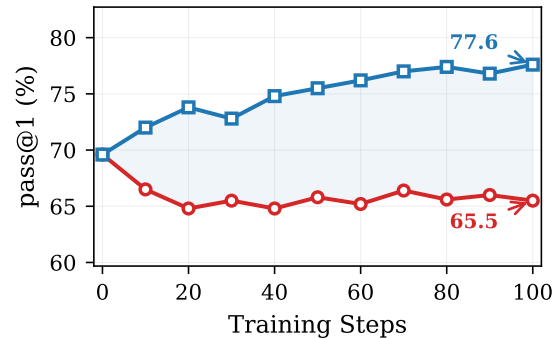
MATH-500
