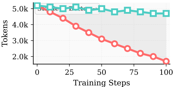
Response Length
