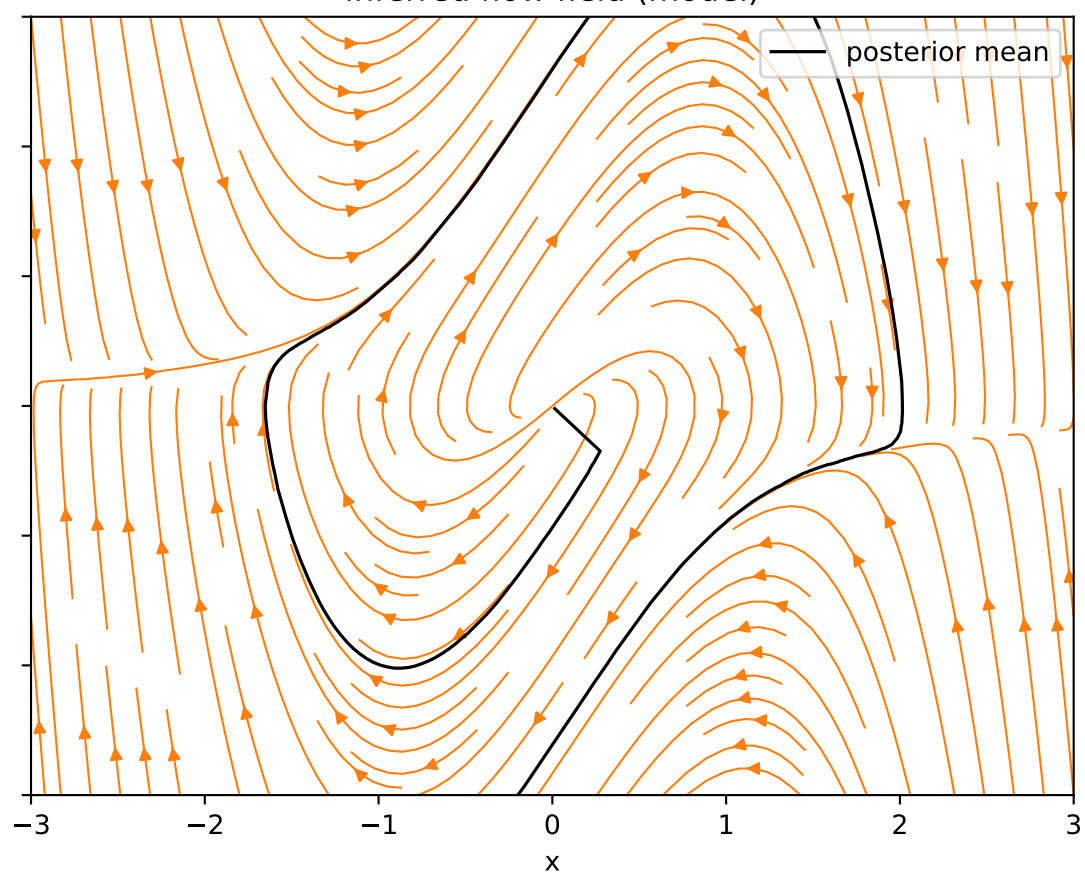
Inferred flow field (model)
