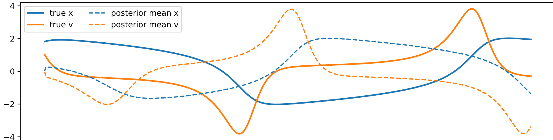
Posterior mean vs true latent (one trial)
