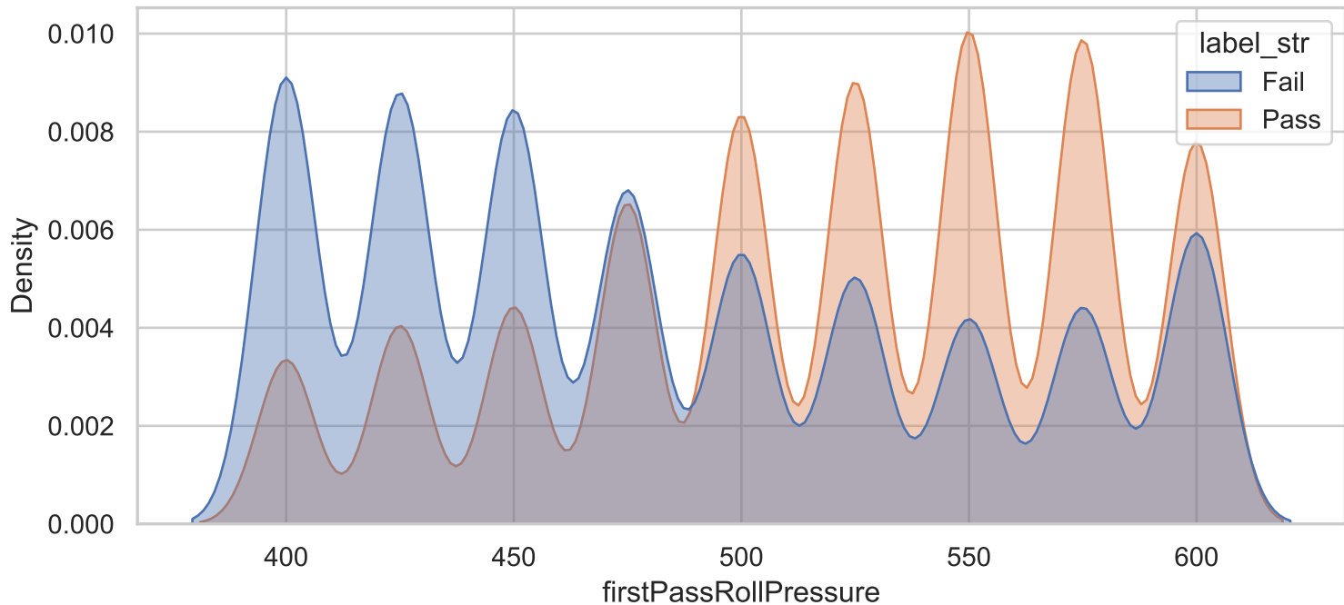
Label Densities for Different Values of firstPassRollPressure
