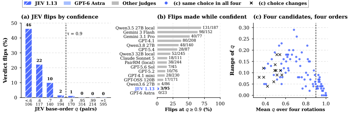
Figure 7: Confidence under presentation order. (a) Share of preference pairs whose JEV verdict changes when the candidates are reversed, by JEV’s base-order confidence q (pairs per bin below the axis); the dashed line marks \tau = 0.9 . (b) For each judge, its reversal flips made at q \geq 0.9 , among flips on pairs with two valid outputs. (c) RewardBench 2, four candidates in four rotations: for each of the 100 prompts, the range of JEV’s confidence across rotations against its mean; crosses mark prompts whose chosen candidate changes between rotations.
