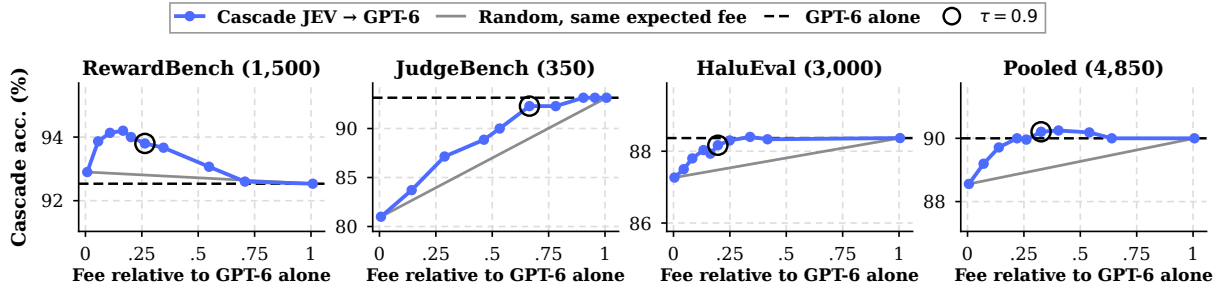
Figure 8: Post hoc confidence cascades JEV→GPT-6 on the base public items. Each curve accepts JEV’s decision when its two-order confidence q \geq \tau and otherwise takes GPT-6’s base-order decision, for \tau \in \{0.5, 0.6, 0.7, 0.8, 0.85, 0.9, 0.95, 0.99, 1\} plus the all-fallback endpoint, against fee relative to GPT-6 alone (reported usage, both JEV orders included); HaluEval answers use JEV’s single judgment. The grey line escalates uniformly at random for the same expected fee, and rings mark \tau = 0.9 . These thresholds are post hoc; Table 3 gives the frozen policies and Appendix Table 28 the numbers.
