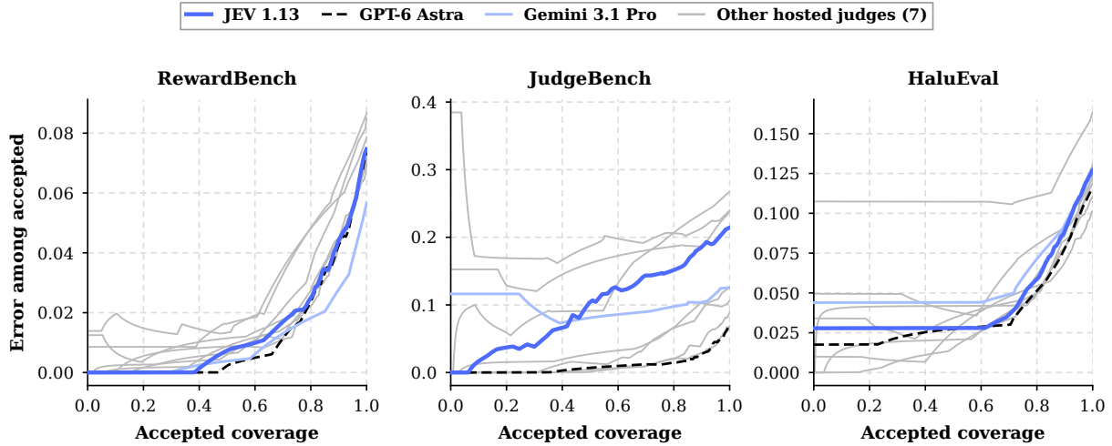
Figure 21: Selective error versus accepted coverage using maximum label probability. Ties use expected within-tie error. These descriptive curves complement the separately evaluated frozen policies.
