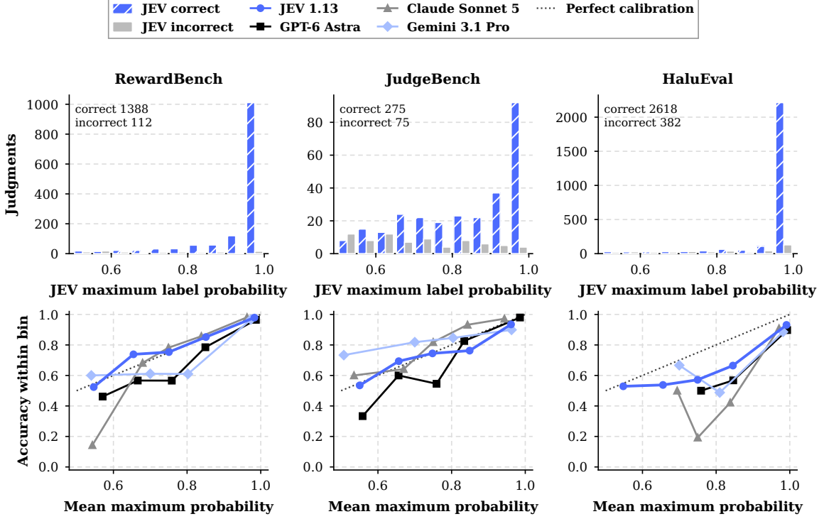
Figure 6: Top: JEV’s maximum-probability distributions for correct and incorrect base judgments, using supplied benchmark labels. Bottom: reliability curves using the same statistic for selected main-round judges (bins with at least five valid examples; full counts retained). Sparse bins, differing coverage, and label errors limit visual ranking; Table 10 gives the HaluEval label sensitivity.
