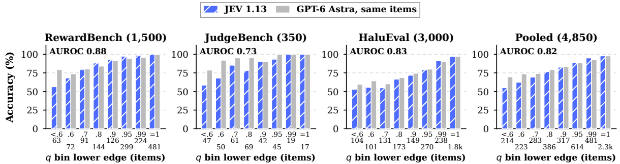
Figure 5: Confidence locates JEV’s errors. JEV judges every preference pair in both orders, and q is its two-order confidence; HaluEval answers have no candidate order and use JEV’s single judgment. Bars give the accuracy of JEV’s decision and of GPT-6’s base-order decision on the same items, binned by q (item counts under the bins; AUROC of q against JEV’s correctness in each panel).
