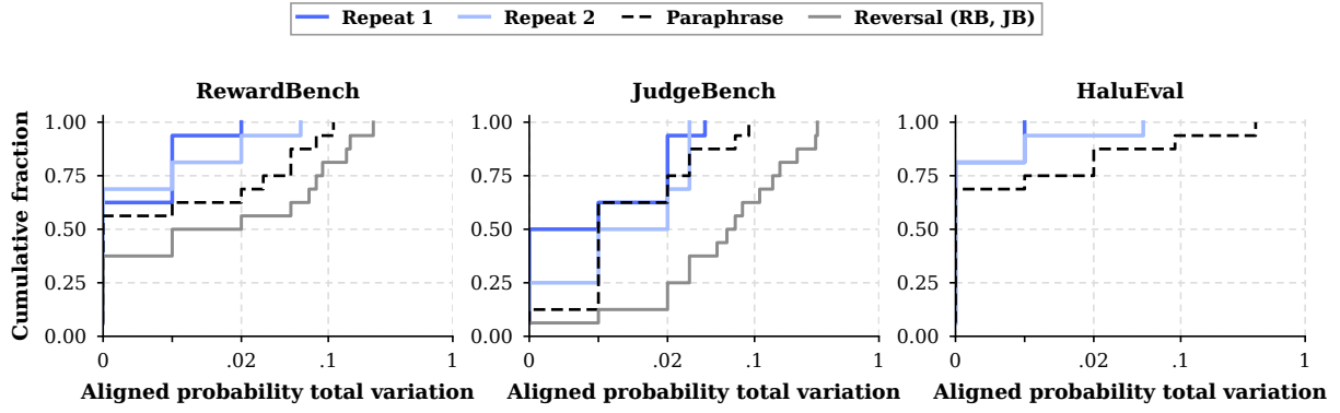
Figure 17: JEV probability variation on the same sixteen examples per task for repetitions, paraphrase, and reversal where applicable. Distributions align semantic response identity. The horizontal scale is linear near zero and logarithmic above 0.02. Full reversal statistics separately use all 1,850 pairs.
