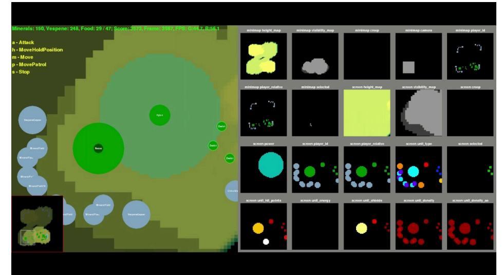
Figure 3: game state is not text. PySC2 exposes StarCraft II as entity and terrain layers (right grid). Serializing this to prose is the naive baseline a learned tokenizer competes against.
