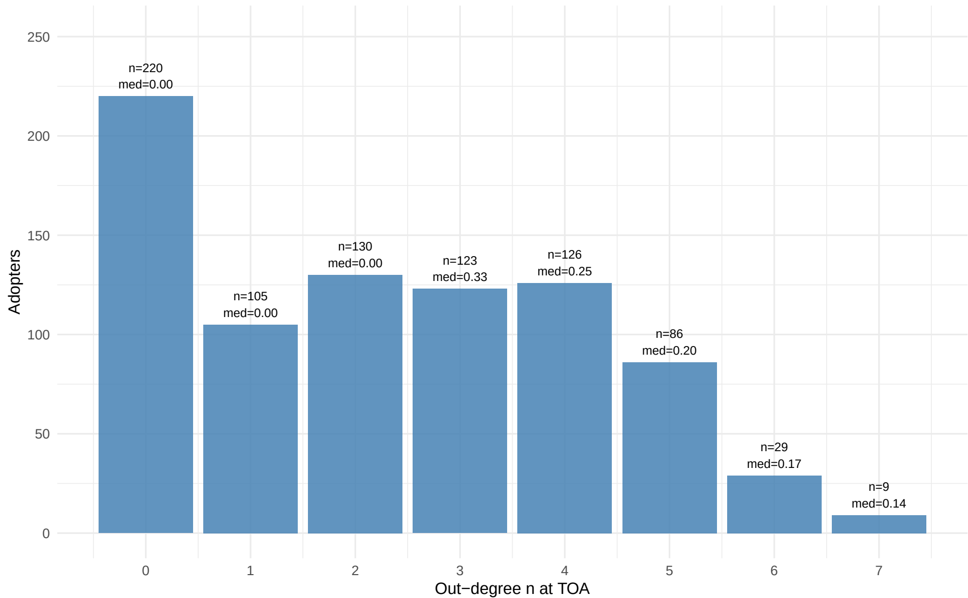
Adopters and median threshold, by out-degree at TOA
